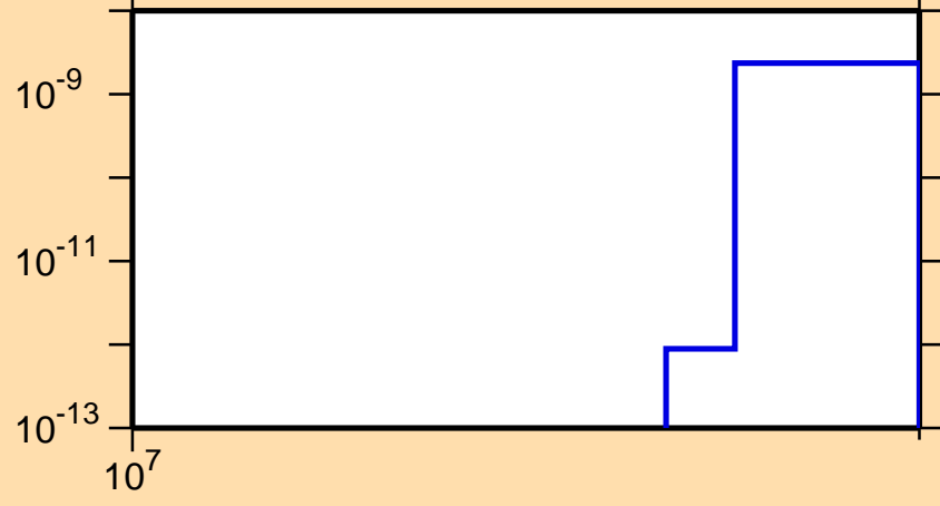
\sigma vs. E for ^{185}\text{Pt}(n,nt)
