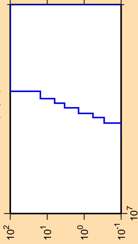
\Delta\sigma/\sigma vs. E for ^{185}\text{Pt}(n,pd)
