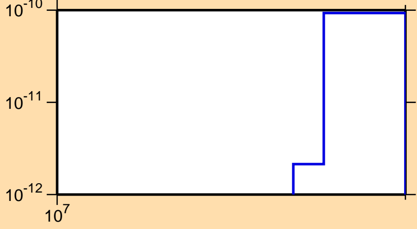
\sigma vs. E for ^{185}\text{Pt} (mt 34)
