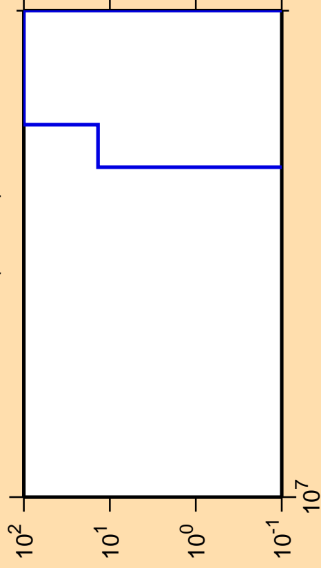
\Delta\sigma/\sigma vs. E for ^{185}\text{Pt} (mt 34)
