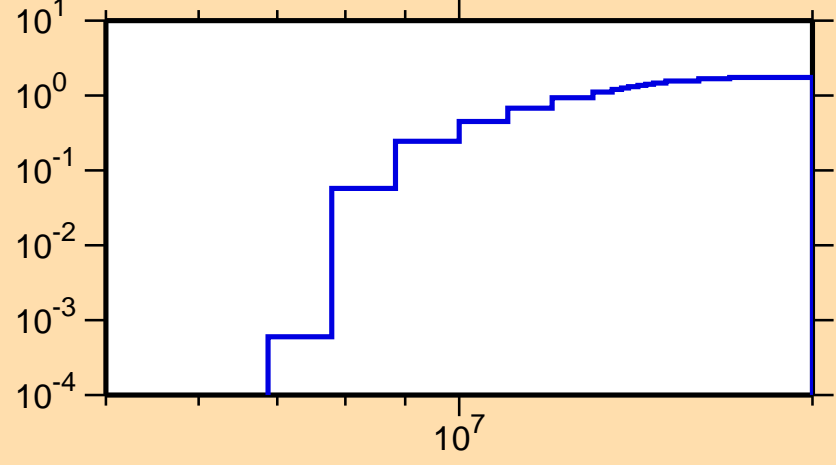
\sigma vs. E for ^{185}\text{Pt}(n,2n)
