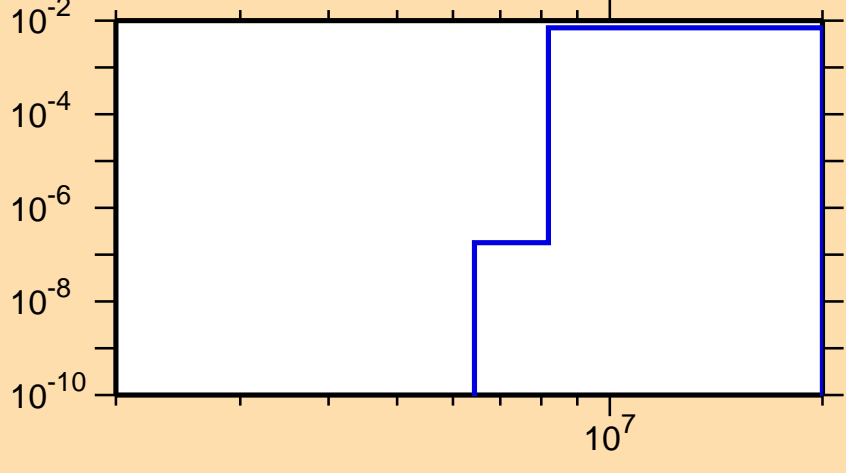
\sigma vs. E for ^{185}\text{Pt}(n,np)
