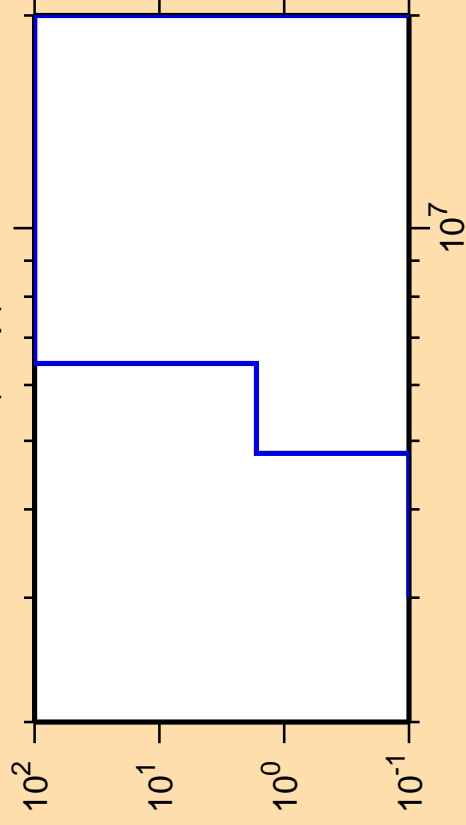
\Delta\sigma/\sigma vs. E for ^{185}\text{Pt}(n,np)
