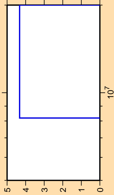
\Delta\sigma/\sigma vs. E for ^{185}\text{Pt}(\text{mt117})
