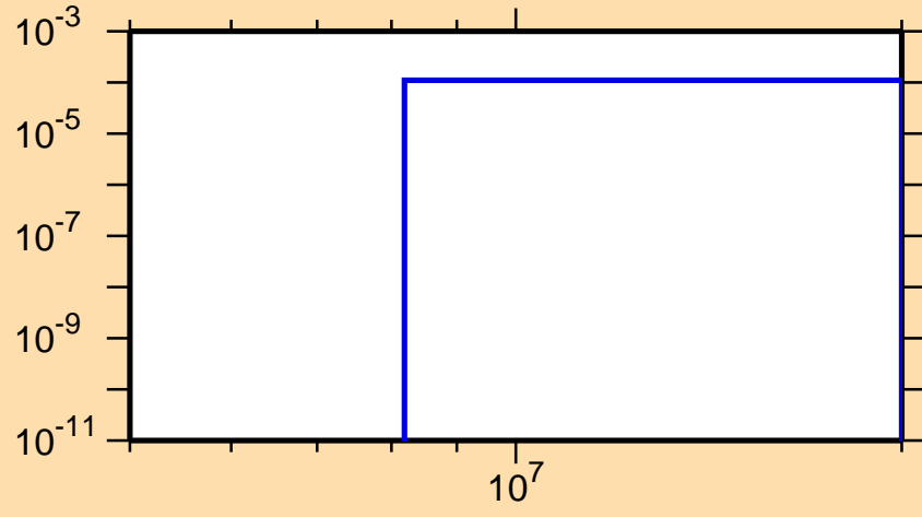
\sigma vs. E for ^{185}\text{Pt}(n,t)
