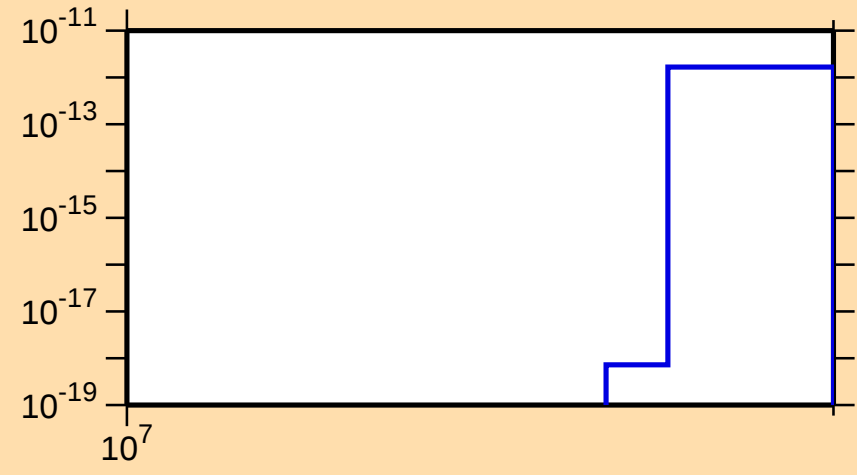
\sigma vs. E for ^{185}\text{Pt}(n,3n\alpha)
