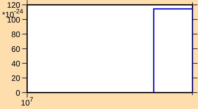
\sigma vs. E for ^{185}\text{Pt}(\text{mt } 11)
