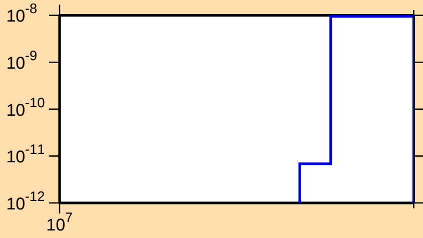
\sigma vs. E for ^{185}\text{Pt}(n,nt)
