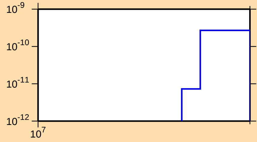
\sigma vs. E for ^{185}\text{Pt}(\text{mt } 34)
