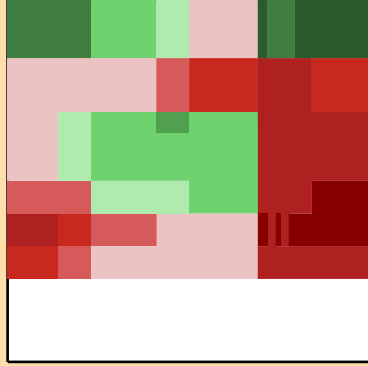
\Delta\sigma/\sigma vs. E for ^{185}\text{Pt}(n,\text{el.})
