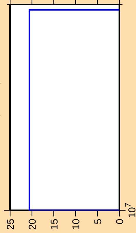
\Delta\sigma/\sigma vs. E for ^{185}\text{Pt}(\text{mt } 34)
