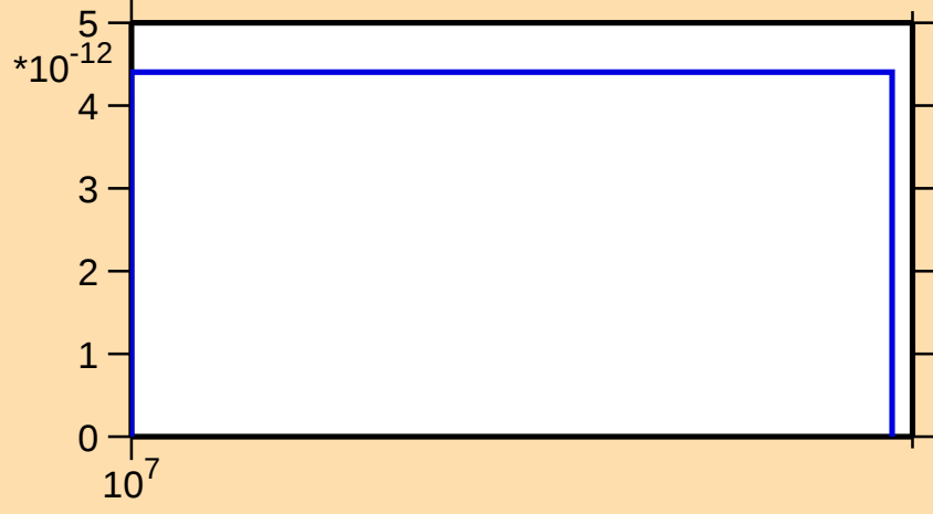
\sigma vs. E for ^{185}\text{Pt}(\text{mt117})
