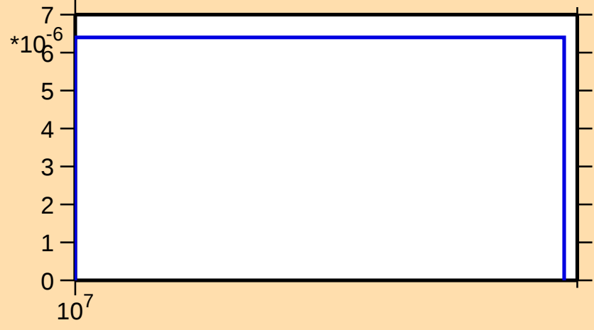
\sigma vs. E for ^{185}\text{Pt}(n,2np)
