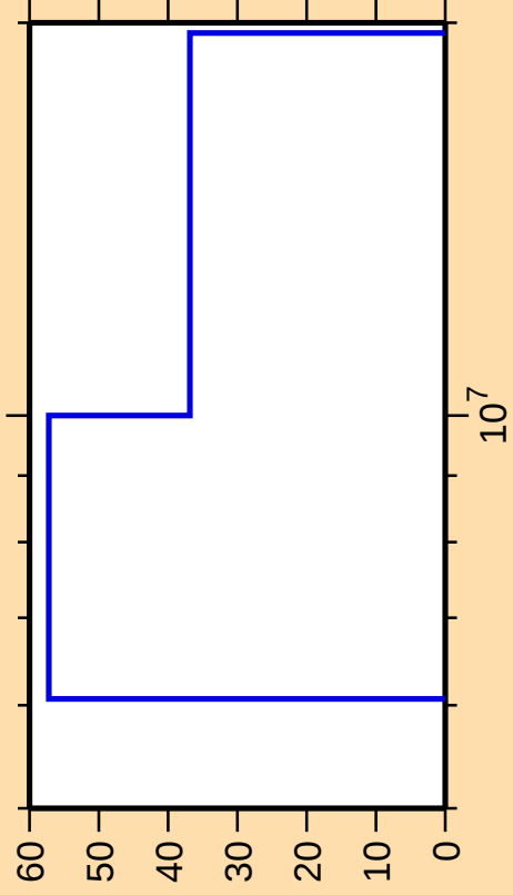
\Delta\sigma/\sigma vs. E for ^{185}\text{Pt}(n,p)
