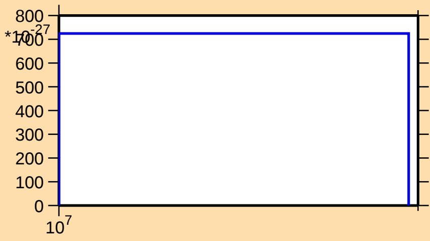
\sigma vs. E for ^{185}\text{Pt}(\text{mt } 11)
