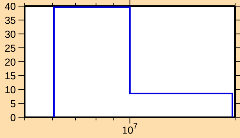
\Delta\sigma/\sigma vs. E for ^{185}\text{Pt}(n,2n)
