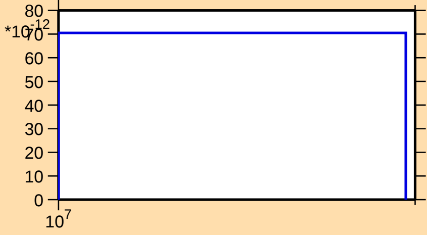
\sigma vs. E for ^{185}\text{Pt}(\text{mt } 45)
