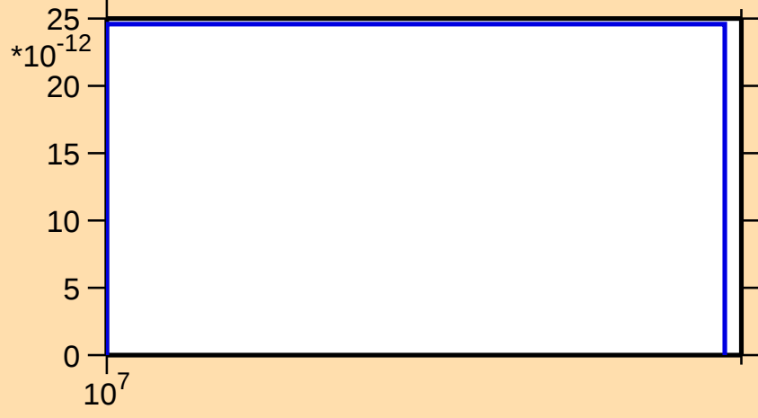
\sigma vs. E for ^{185}\text{Pt}(n,\text{pt})
