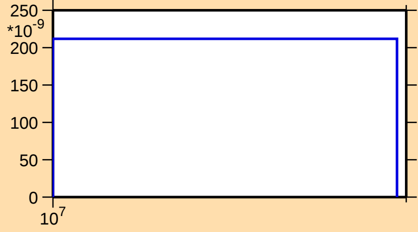
\sigma vs. E for ^{185}\text{Pt}(n,\text{nd})
