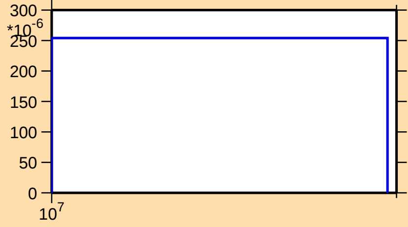
\sigma vs. E for ^{185}\text{Pt}(n,3n)
