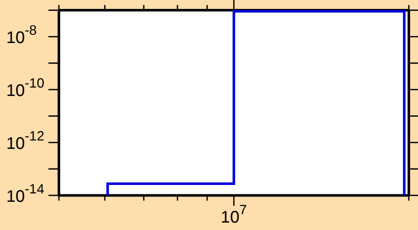
\sigma vs. E for ^{185}\text{Pt}(n,\text{He3})
