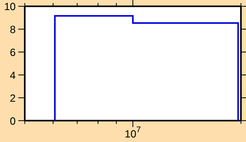
\Delta\sigma/\sigma vs. E for ^{185}\text{Pt}(n,\text{nonel.})
