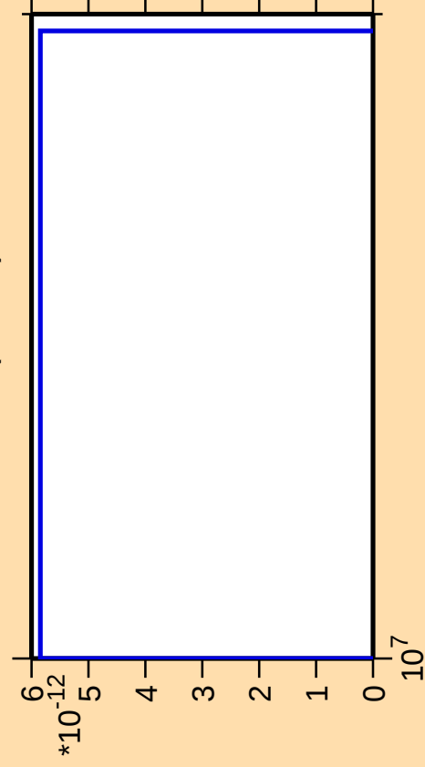
\Delta\sigma/\sigma vs. E for ^{185}\text{Pt}(\text{mt } 11)
