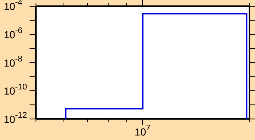
\sigma vs. E for ^{185}\text{Pt}(n,2n\alpha)
