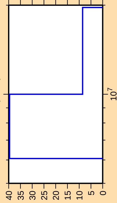
\Delta\sigma/\sigma vs. E for ^{185}\text{Pt}(n,2n)
