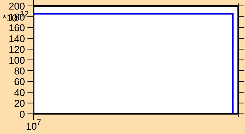
\sigma vs. E for ^{185}\text{Pt}(n,\text{pd})
