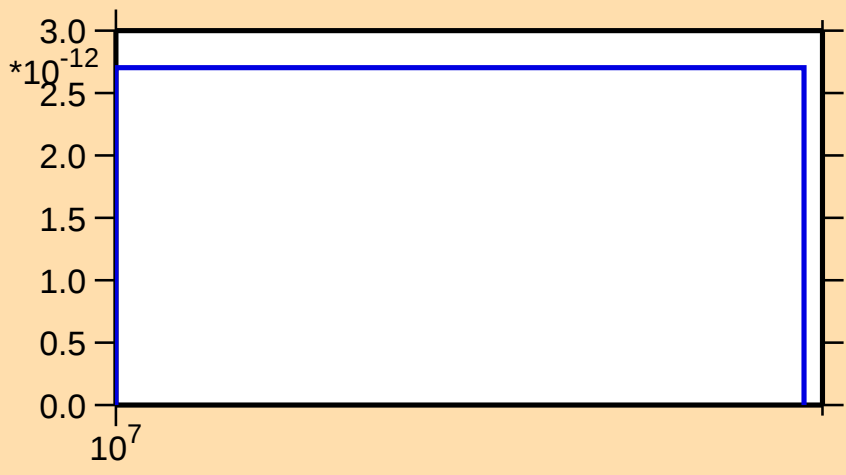
\sigma vs. E for ^{185}\text{Pt}(\text{mt } 34)
