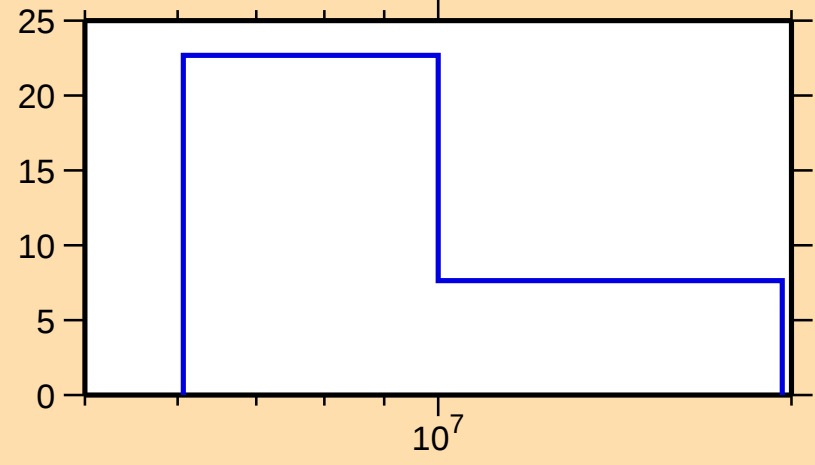
\Delta\sigma/\sigma vs. E for ^{185}\text{Pt}(n,\text{tot.})
