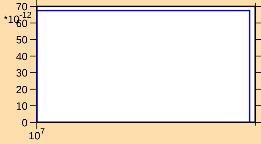
\sigma vs. E for ^{185}\text{Pt}(n,nt)
