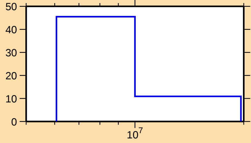
\Delta\sigma/\sigma vs. E for ^{185}\text{Pt}(n,\text{el.})
