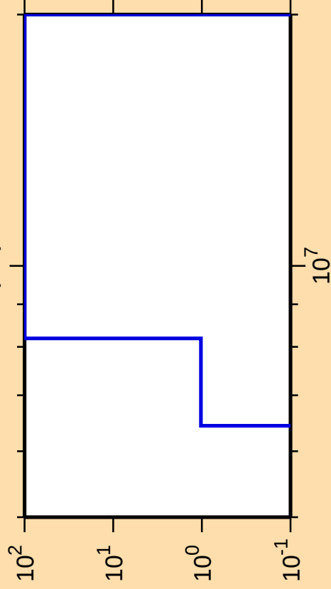
\Delta\sigma/\sigma vs. E for ^{185}\text{Pt}(n,t)
