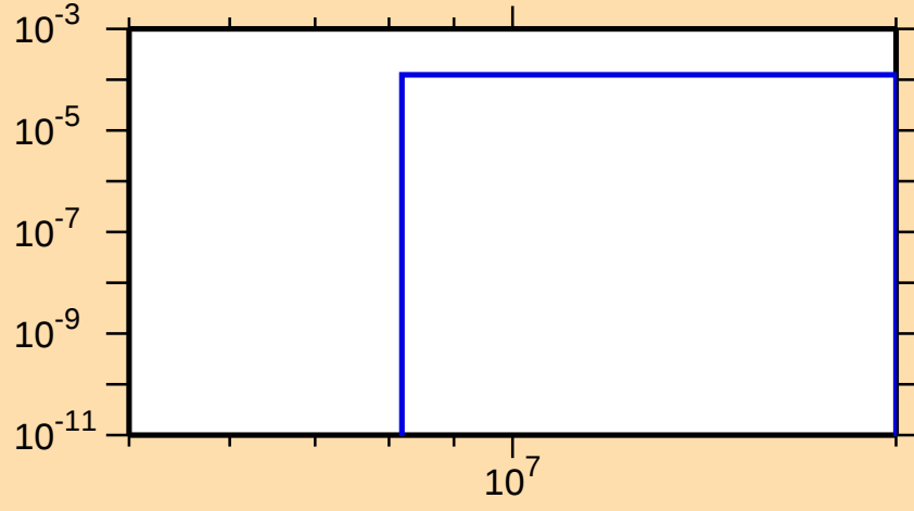
\sigma vs. E for ^{185}\text{Pt}(n,t)
