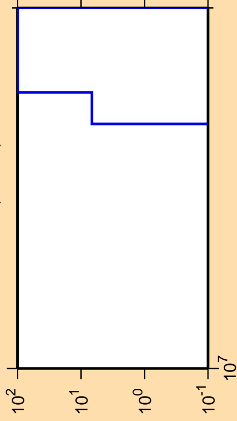
\Delta\sigma/\sigma vs. E for ^{187}\text{Pt} (mt 34)
