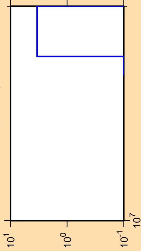
\Delta\sigma/\sigma vs. E for ^{187}\text{Pt}(n,3n\alpha)
