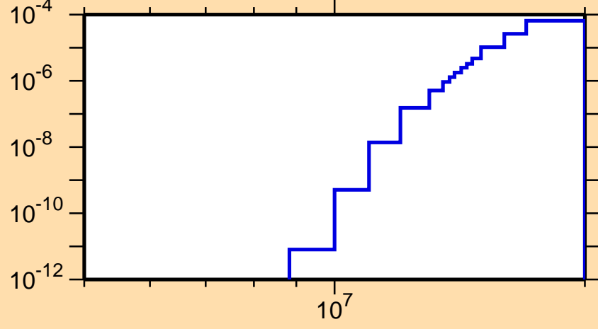
\sigma vs. E for ^{187}\text{Pt}(n,2n\alpha)
