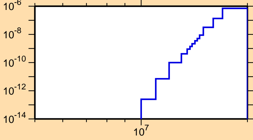
\sigma vs. E for ^{187}\text{Pt}(n,\text{He}3)
