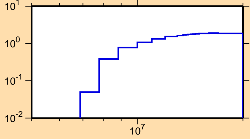
\sigma vs. E for ^{187}\text{Pt}(n,2n)
