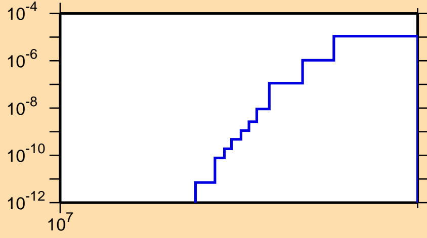
\sigma vs. E for ^{187}\text{Pt}(n,\text{nd})
