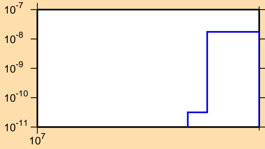
\sigma vs. E for ^{187}\text{Pt}(n,nt)
