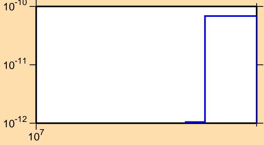
\sigma vs. E for ^{187}\text{Pt} (mt 34)
