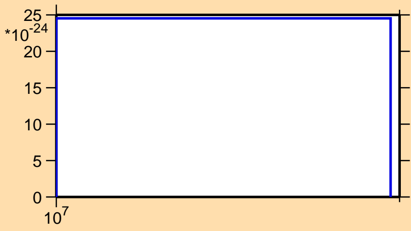
\sigma vs. E for ^{187}\text{Pt}(\text{mt } 11)
