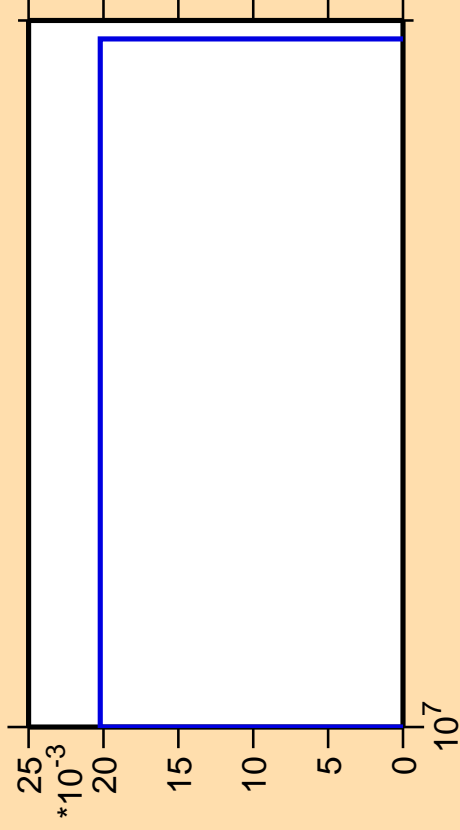
\Delta\sigma/\sigma vs. E for ^{187}\text{Pt}(n,3n\alpha)
