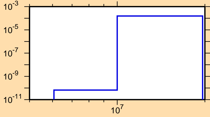
\sigma vs. E for ^{187}\text{Pt}(n,t)
