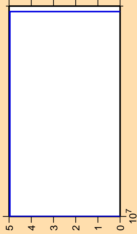
\Delta\sigma/\sigma vs. E for ^{187}\text{Pt}(n,\text{pt})
