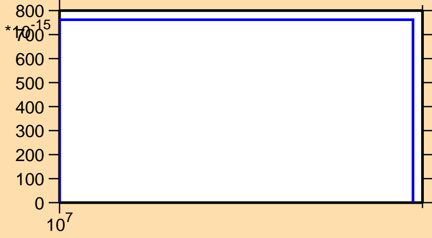
\sigma vs. E for ^{187}\text{Pt}(n,\text{pt})
