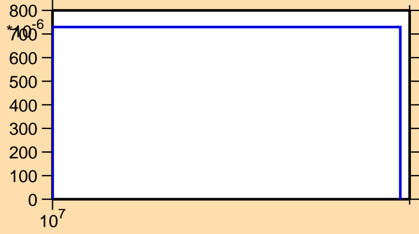
\sigma vs. E for ^{187}\text{Pt}(n,3n)
