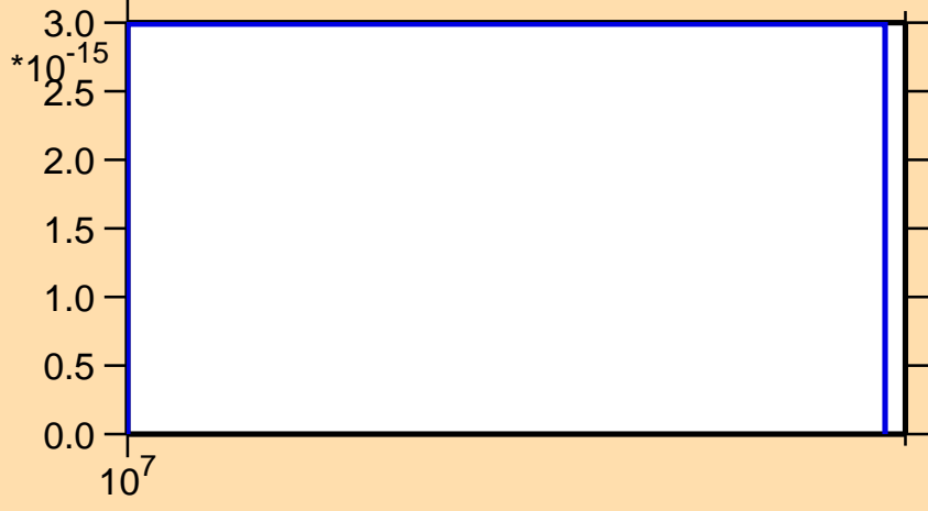
\sigma vs. E for ^{187}\text{Pt}(n,3n\alpha)
