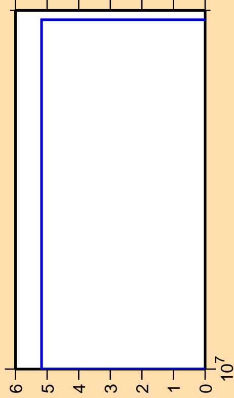
\Delta\sigma/\sigma vs. E for ^{187}\text{Pt}(n,\text{pd})
