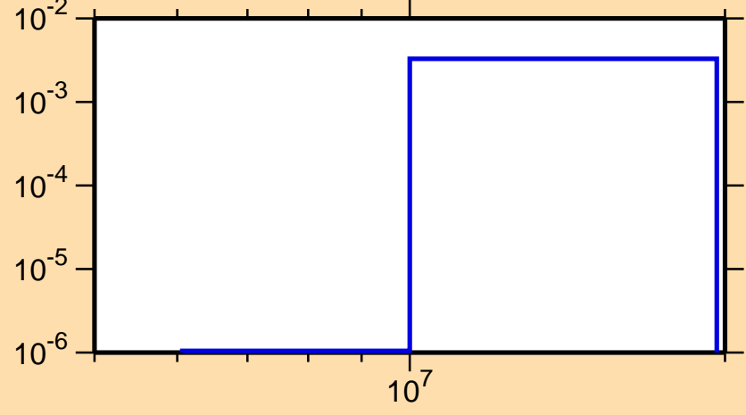
\sigma vs. E for ^{187}\text{Pt}(n,np)
