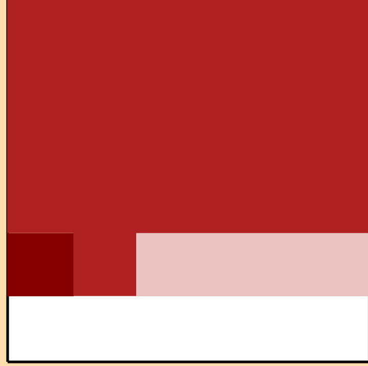
\Delta\sigma/\sigma vs. E for ^{187}\text{Pt}(n,\text{el.})
