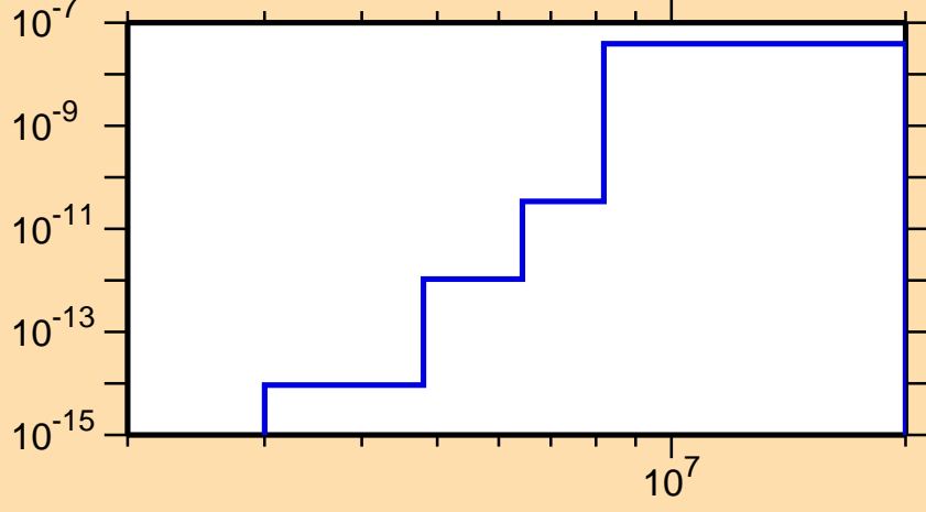
\sigma vs. E for ^{187}\text{Pt}(n,p\alpha)
