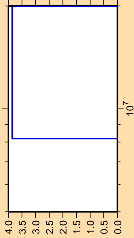
\Delta\sigma/\sigma vs. E for ^{187}\text{Pt}(\text{mt } 34)
