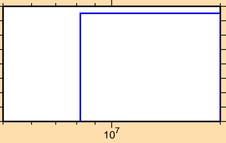
\sigma vs. E for ^{187}\text{Pt}(n,2n\alpha)
