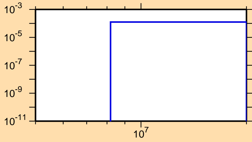
\sigma vs. E for ^{187}\text{Pt}(n,t)
