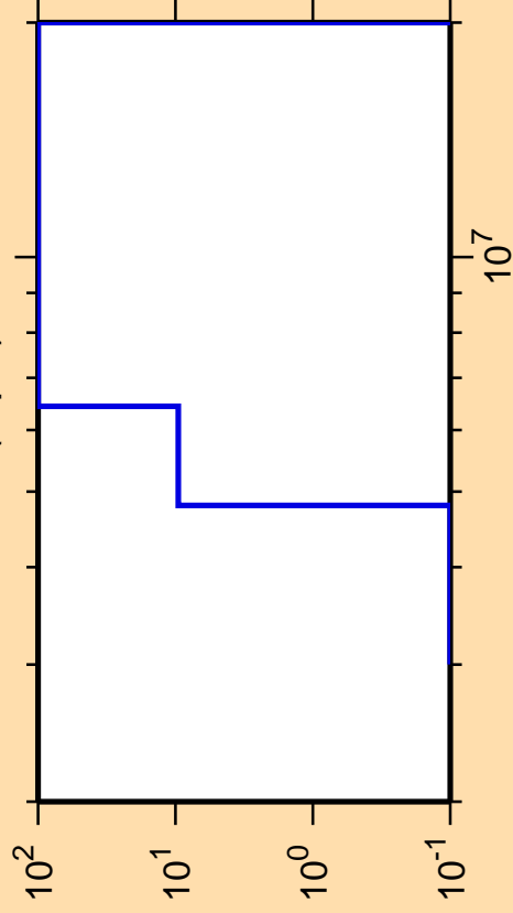
\Delta\sigma/\sigma vs. E for ^{187}\text{Pt}(n,p\alpha)
