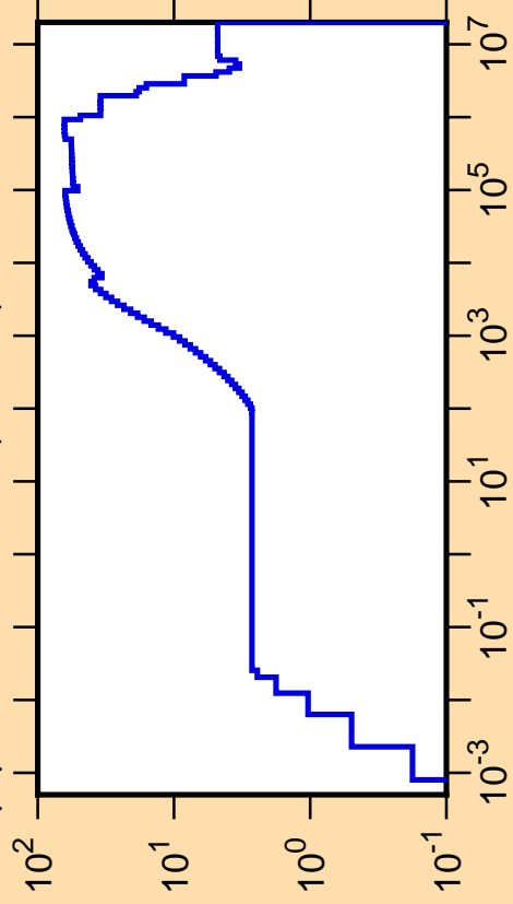
\Delta\mu/\mu vs. E for ^{188}\text{Pt}(\text{mt251})
