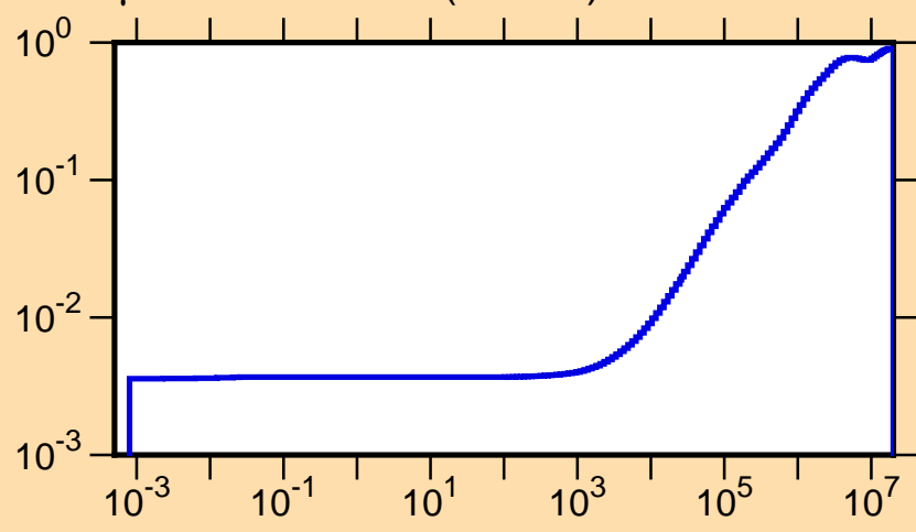
\mu vs. E for ^{188}\text{Pt}(\text{mt251})
