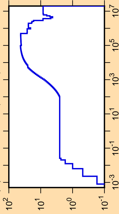
\Delta\mu/\mu vs. E for ^{189}\text{Pt}(\text{mt251})
