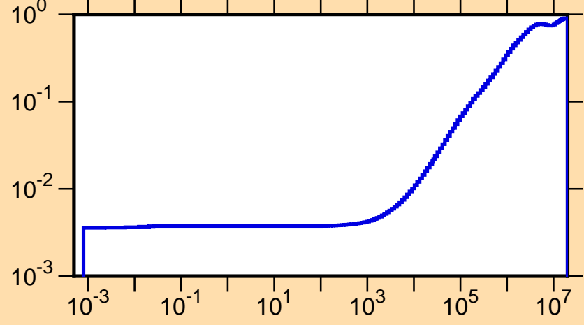
\mu vs. E for ^{189}\text{Pt}(\text{mt251})
