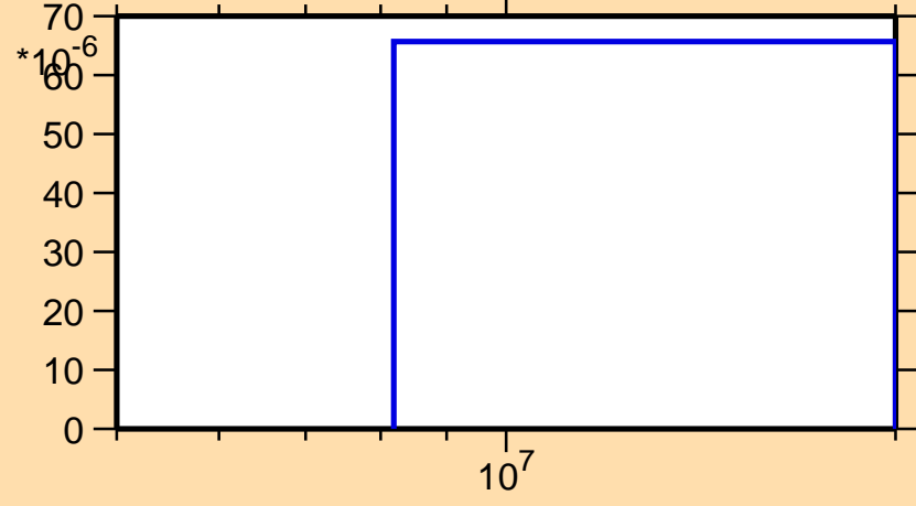
\sigma vs. E for ^{189}\text{Pt}(n,t)
