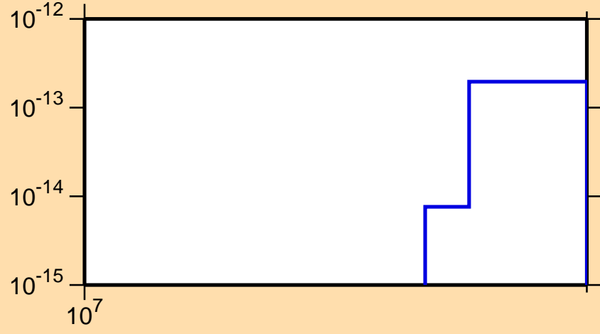
\sigma vs. E for ^{190}\text{Pt(mt117)}
