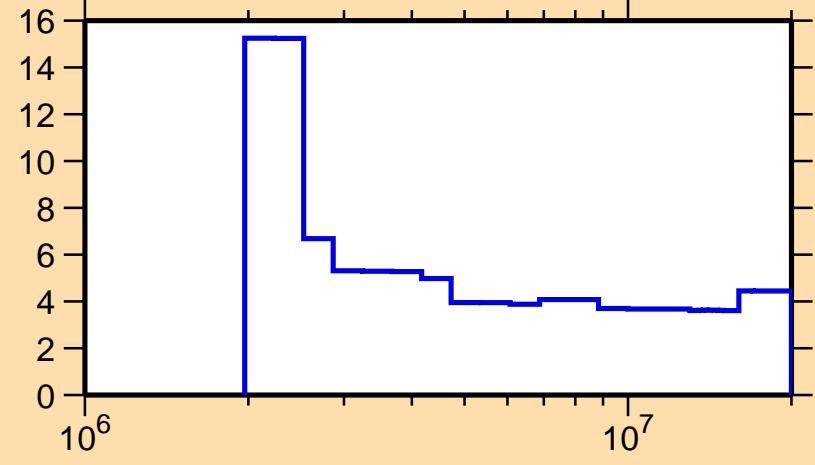
\Delta\sigma/\sigma vs. E for ^{190}\text{Pt}(n,n\text{onel.})
