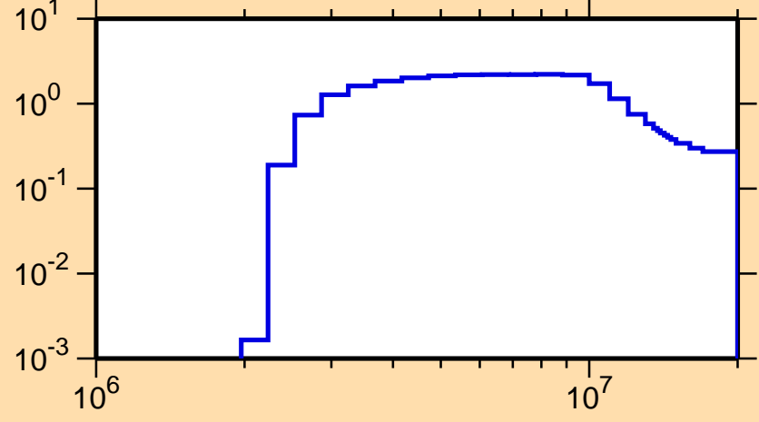
\sigma vs. E for ^{190}\text{Pt}(n,n\text{cont.})
