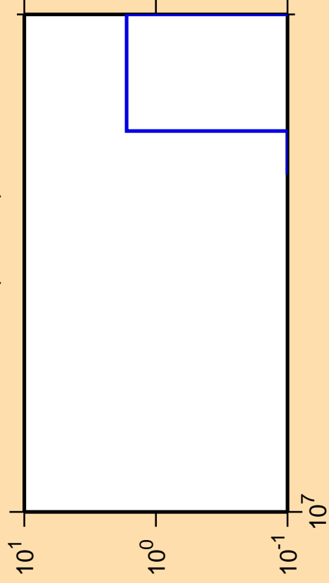
\Delta\sigma/\sigma vs. E for ^{190}\text{Pt(mt117)}
