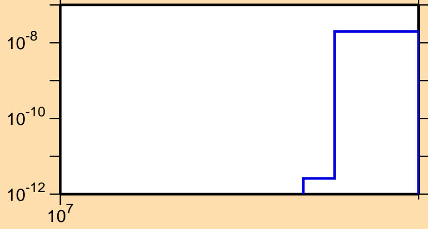
\sigma vs. E for ^{190}\text{Pt}(n,2np)
