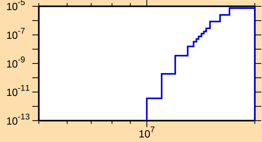
\sigma vs. E for ^{191}\text{Pt}(n,2n\alpha)
