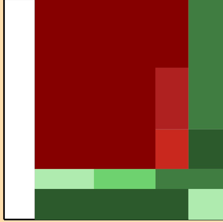
\Delta\sigma/\sigma vs. E for ^{191}\text{Pt}(n,2n)
