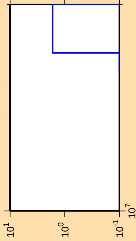
\Delta\sigma/\sigma vs. E for ^{191}\text{Pt}(n,3n\alpha)
