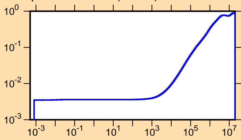
\mu vs. E for ^{193}\text{Pt}(\text{mt251})
