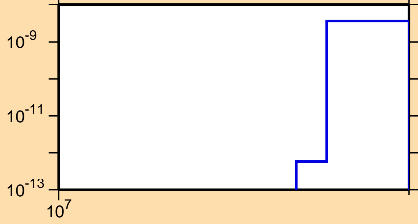
\sigma vs. E for ^{193}\text{Pt}(n,nt)
