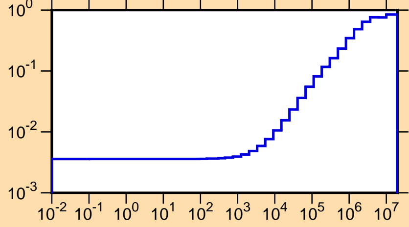
\mu vs. E for ^{193}\text{Pt}(\text{mt251})
