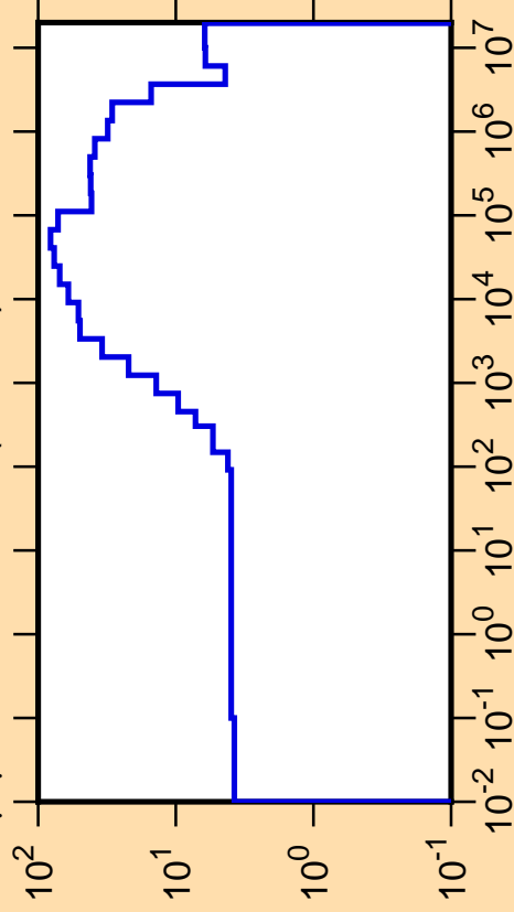
\Delta\mu/\mu vs. E for ^{193}\text{Pt}(\text{mt251})
