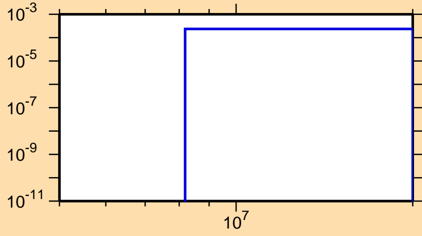
\sigma vs. E for ^{193}\text{Pt}(n,d)
