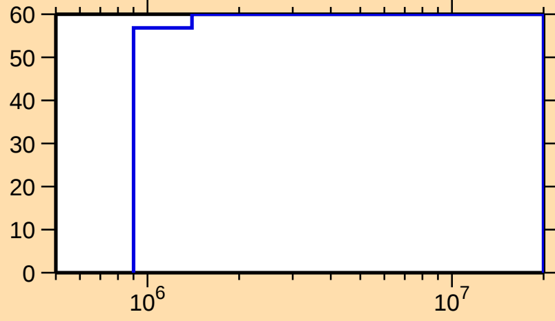
\Delta\sigma/\sigma vs. E for ^{193}\text{Pt}(n,\gamma)
