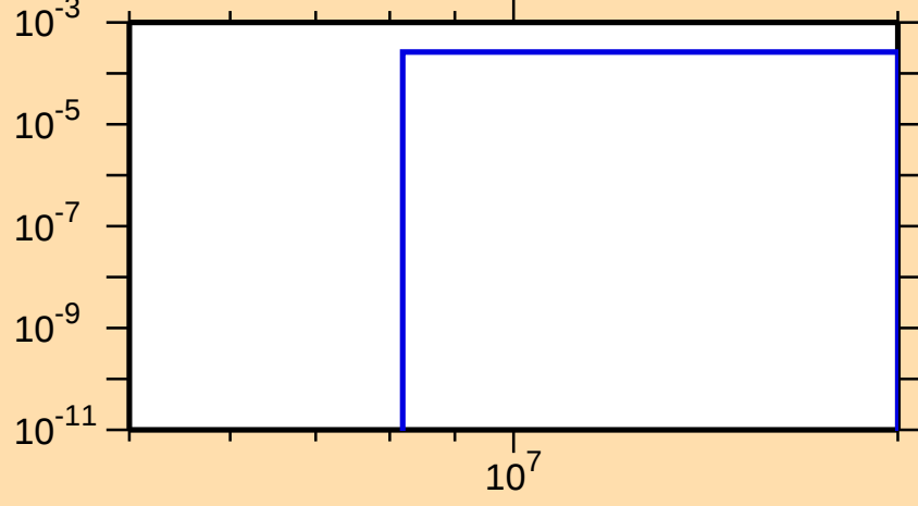
\sigma vs. E for ^{193}\text{Pt}(n,d)
