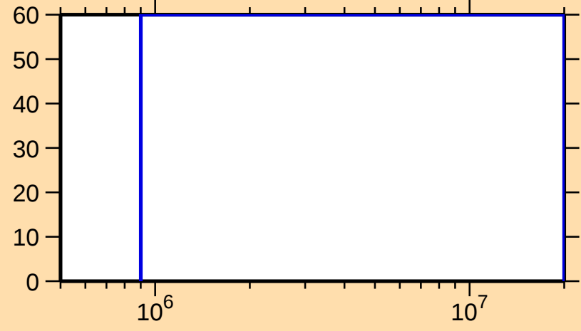
\Delta\sigma/\sigma vs. E for ^{193}\text{Pt}(n,n_1)
