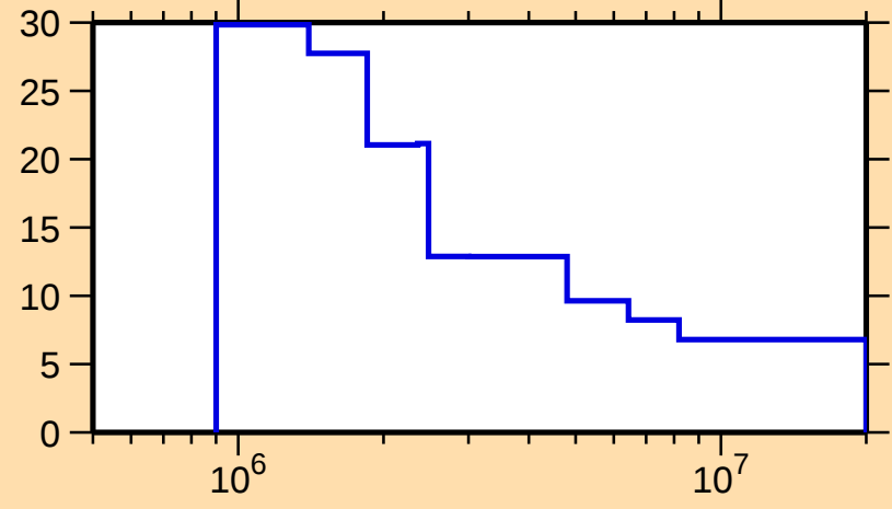
\Delta\sigma/\sigma vs. E for ^{193}\text{Pt}(n,\text{nonel.})
