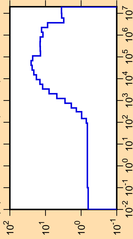
\Delta\mu/\mu vs. E for ^{194}\text{Pt}(\text{mt251})
