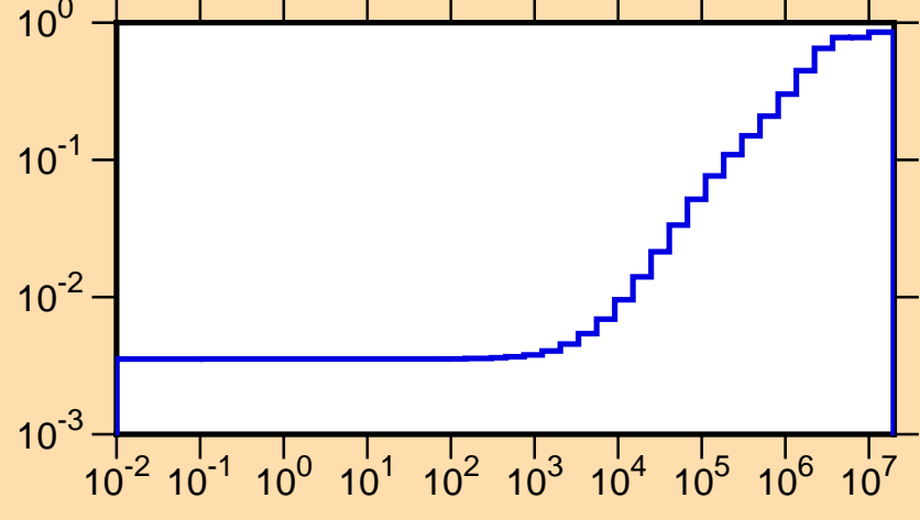
\mu vs. E for ^{194}\text{Pt}(\text{mt251})
