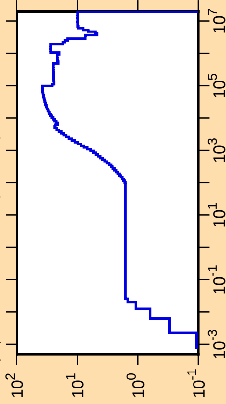
\Delta\mu/\mu vs. E for ^{195}\text{Pt}(\text{mt251})
