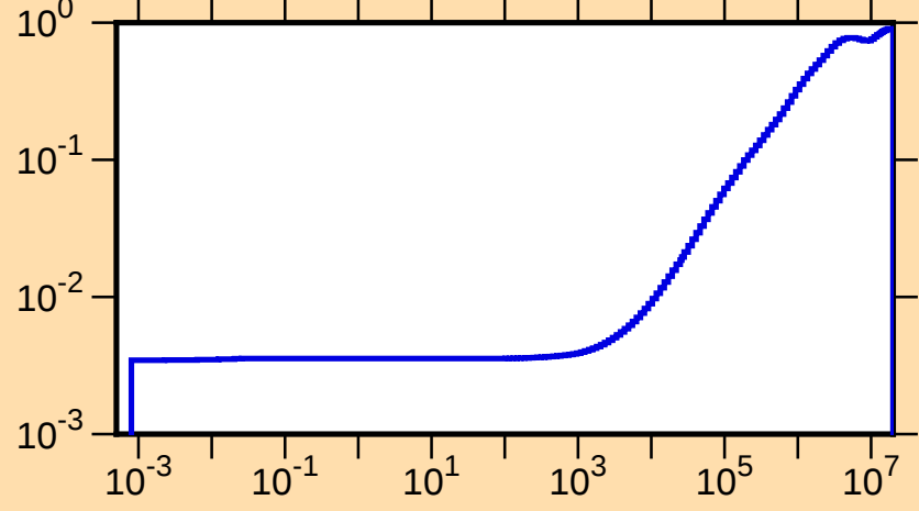
\mu vs. E for ^{195}\text{Pt}(\text{mt251})
