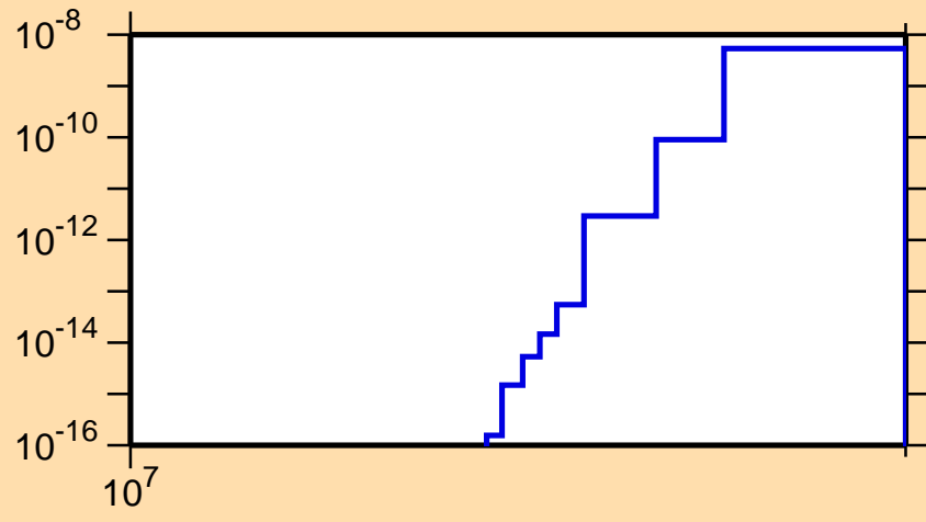
\sigma vs. E for ^{196}\text{Pt}(n,2n\alpha)
