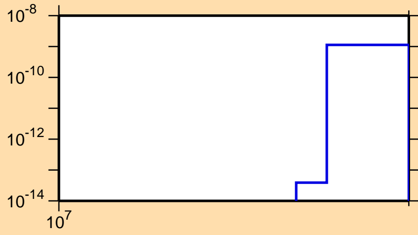
\sigma vs. E for ^{196}\text{Pt}(n,nt)
