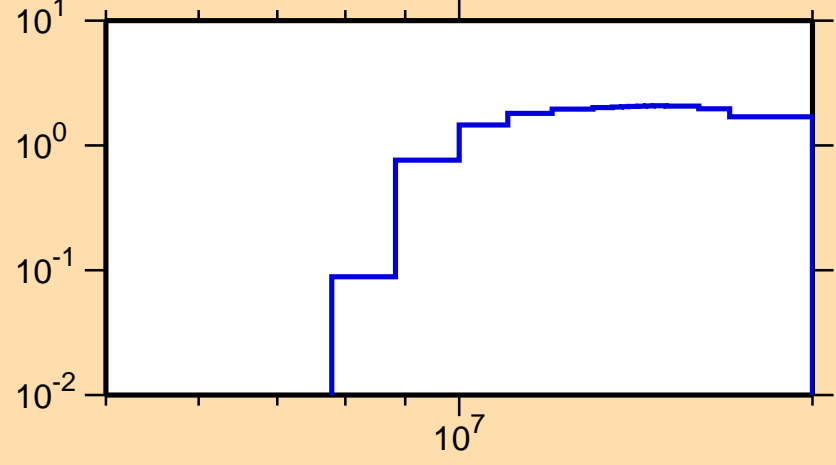
\sigma vs. E for ^{196}\text{Pt}(n,2n)
