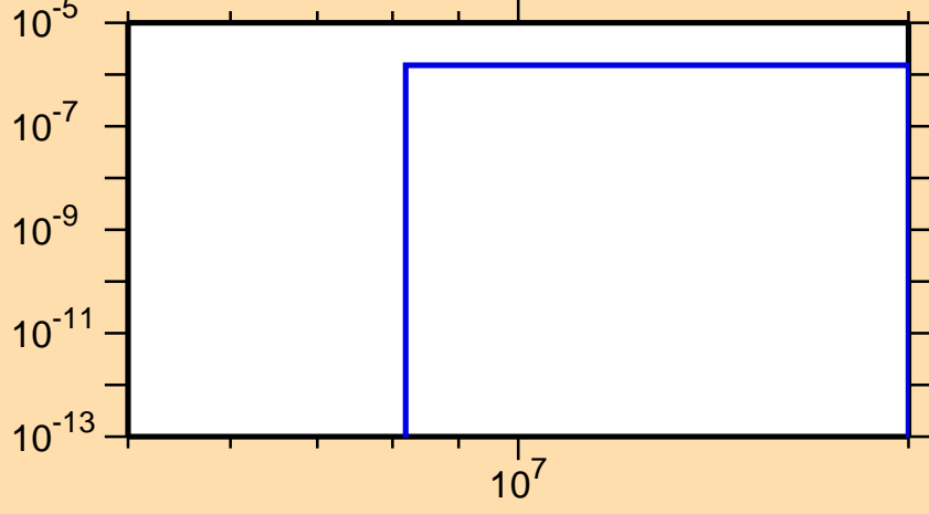
\sigma vs. E for ^{197}\text{Pt}(n,\alpha)
