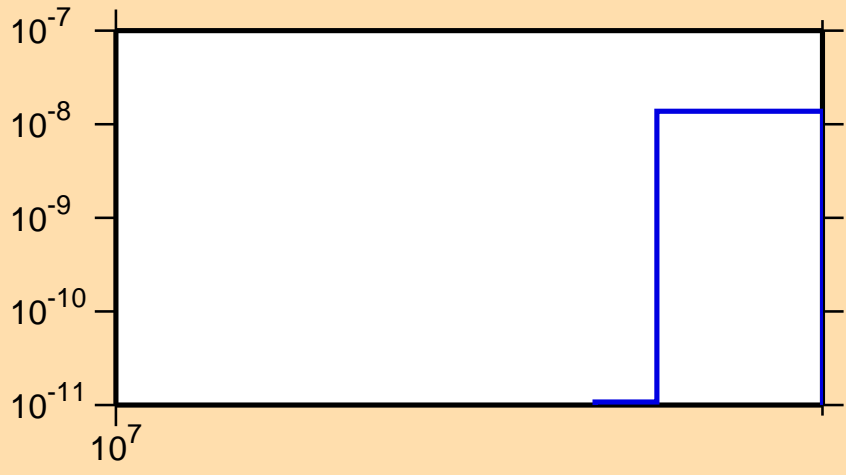
\sigma vs. E for ^{197}\text{Pt}(n,2np)
