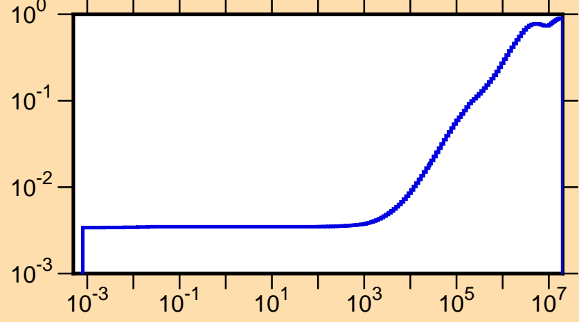
\mu vs. E for ^{198}\text{Pt}(\text{mt251})
