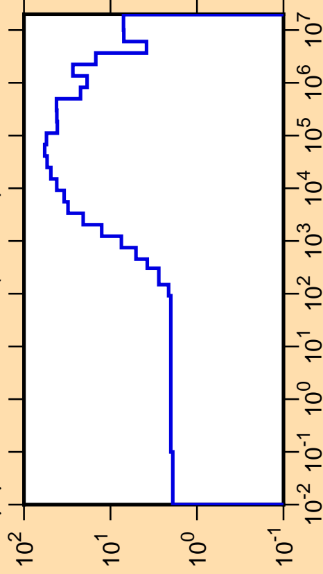
\Delta\mu/\mu vs. E for ^{198}\text{Pt}(\text{mt251})
