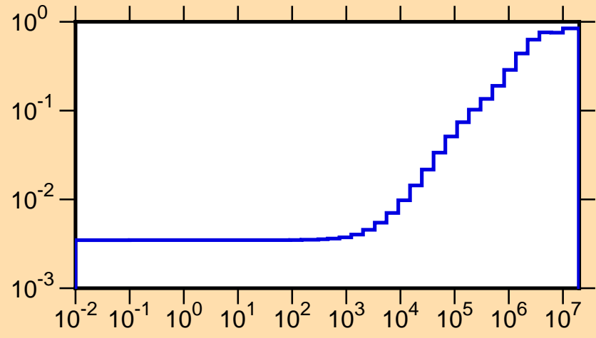
\mu vs. E for ^{198}\text{Pt}(\text{mt251})
