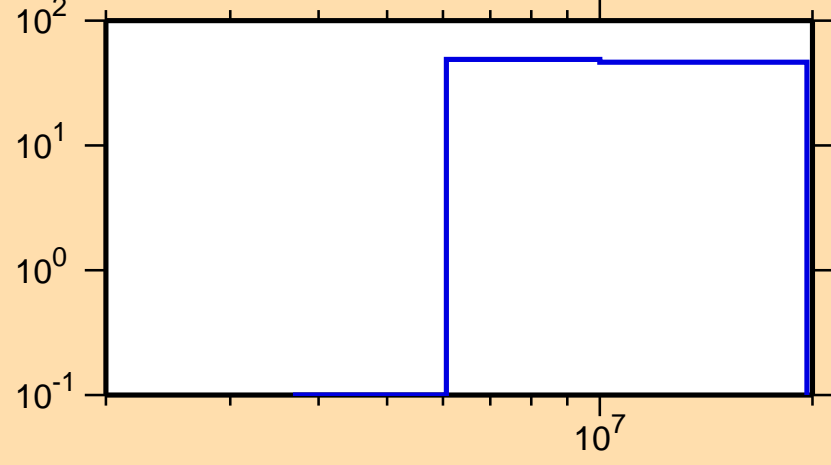
\Delta\sigma/\sigma vs. E for ^{198}\text{Pt}(n,p)
