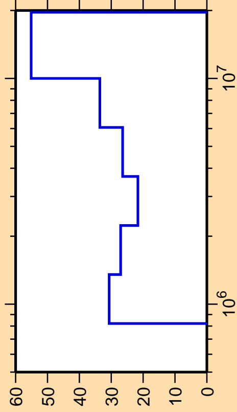
\Delta\sigma/\sigma vs. E for ^{198}\text{Pt}(n,n_3)
