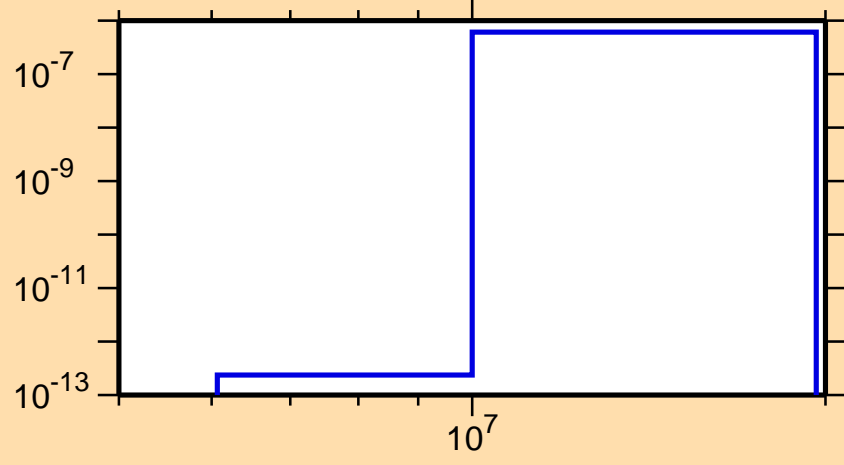
\sigma vs. E for ^{198}\text{Pt}(n,n\alpha)
