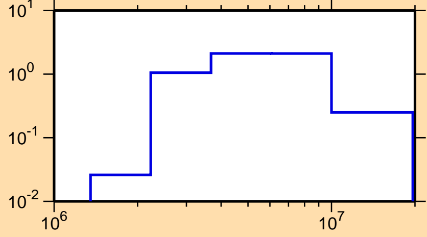
\sigma vs. E for ^{198}\text{Pt}(n,n\text{cont.})
