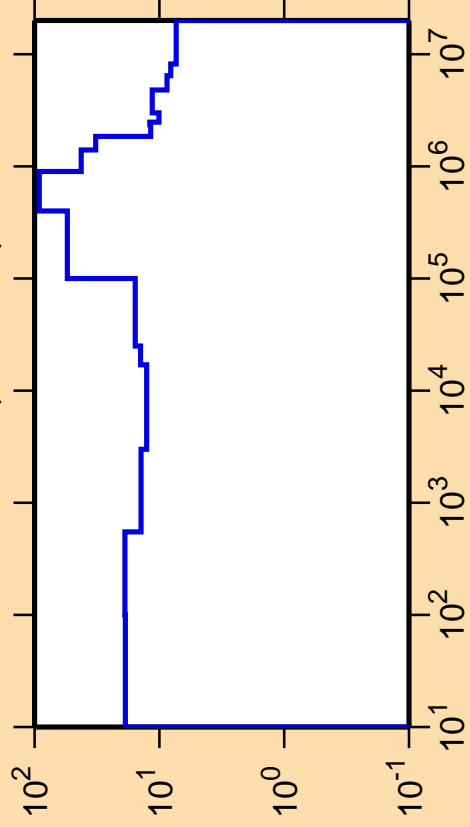
\Delta\sigma/\sigma vs. E for ^{198}\text{Pt}(n,\text{nonel.})
