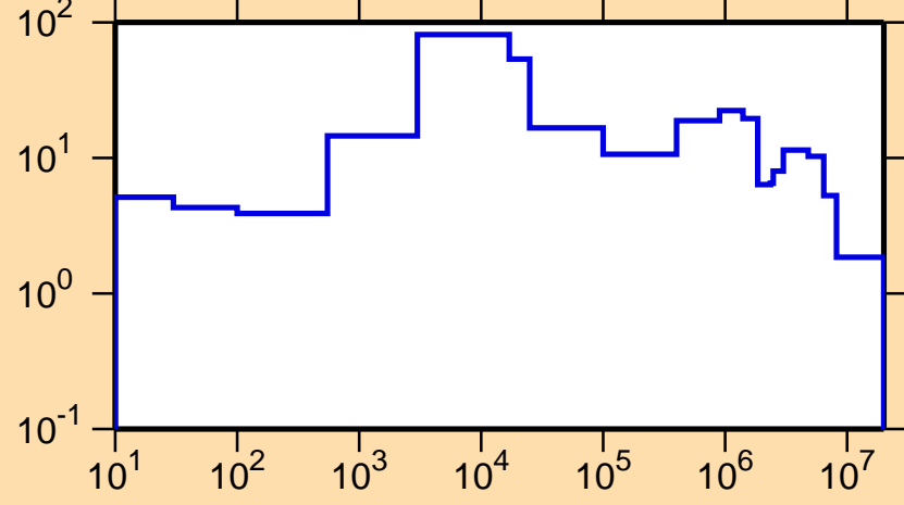
\Delta\sigma/\sigma vs. E for ^{198}\text{Pt}(n,\text{tot.})
