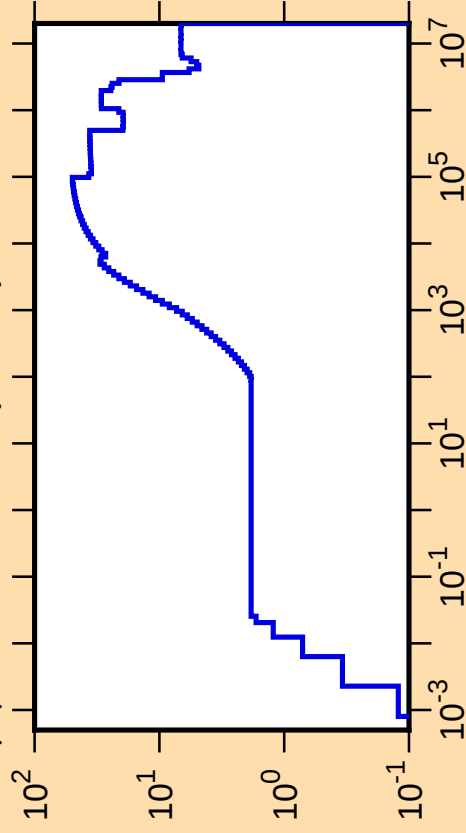
\Delta\mu/\mu vs. E for ^{199}\text{Pt}(\text{mt251})
