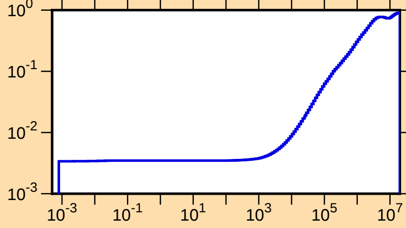
\mu vs. E for ^{199}\text{Pt}(\text{mt251})
