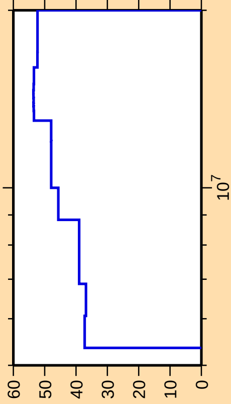
\Delta\sigma/\sigma vs. E for ^{199}\text{Pt}(n,\gamma)
