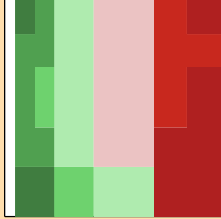
\Delta\sigma/\sigma vs. E for ^{199}\text{Pt}(n,2n)
