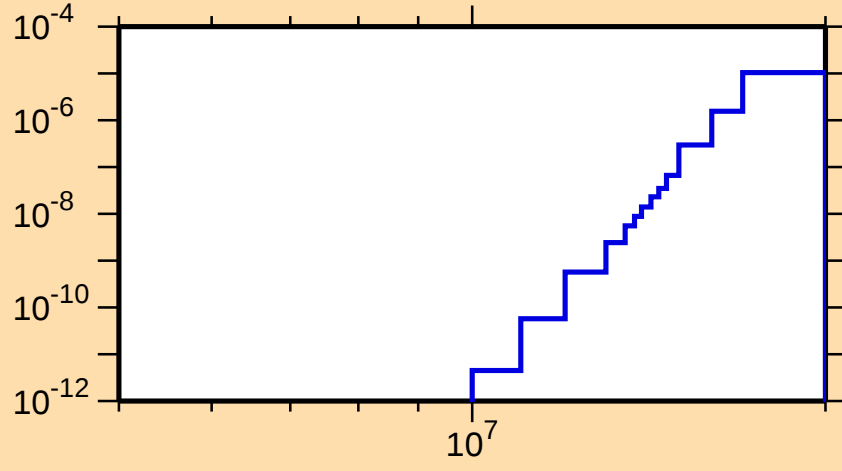
\sigma vs. E for ^{199}\text{Pt}(n,\alpha)
