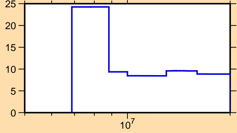
\Delta\sigma/\sigma vs. E for ^{200}\text{Pt}(n,\text{el.})
