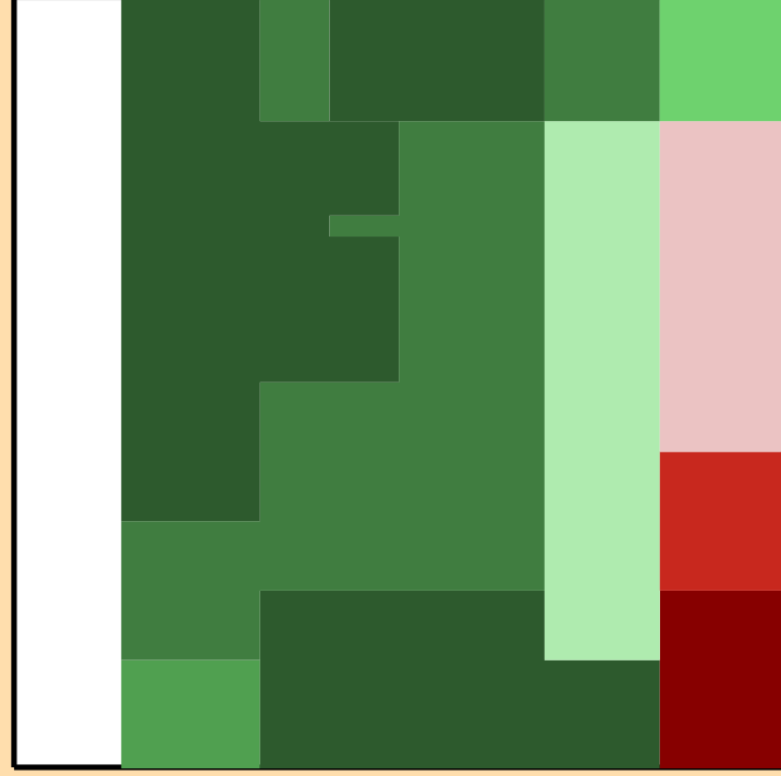
\Delta\sigma/\sigma vs. E for ^{200}\text{Pt}(n,p)
