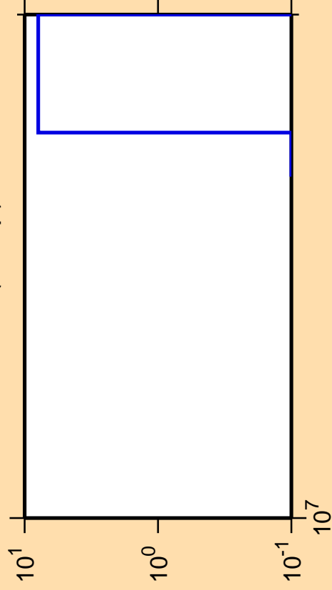
\Delta\sigma/\sigma vs. E for ^{200}\text{Pt}(n,2np)
