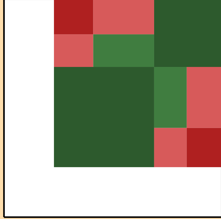
\sigma vs. E for ^{200}\text{Pt}(n,2n)
