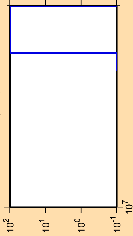
\Delta\sigma/\sigma vs. E for ^{200}\text{Pt}(n,nt)
