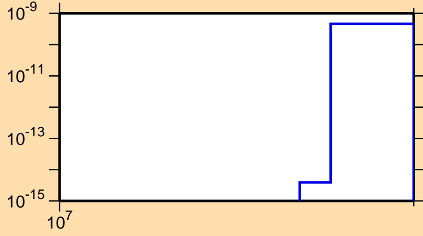
\sigma vs. E for ^{200}\text{Pt}(n,nt)
