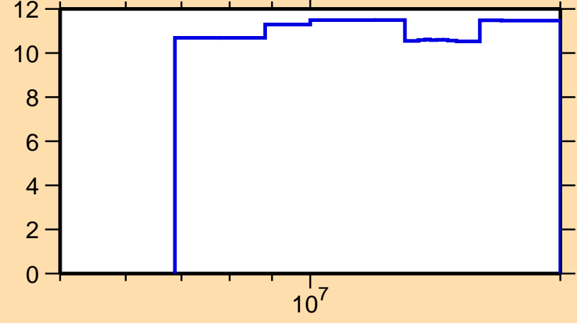
\Delta\sigma/\sigma vs. E for ^{200}\text{Pt}(n,\text{nonel.})
