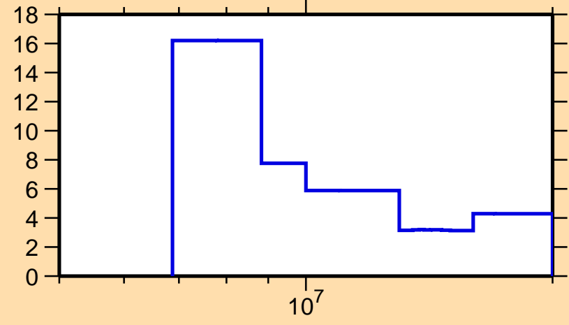
\Delta\sigma/\sigma vs. E for ^{200}\text{Pt}(n,\text{tot.})
