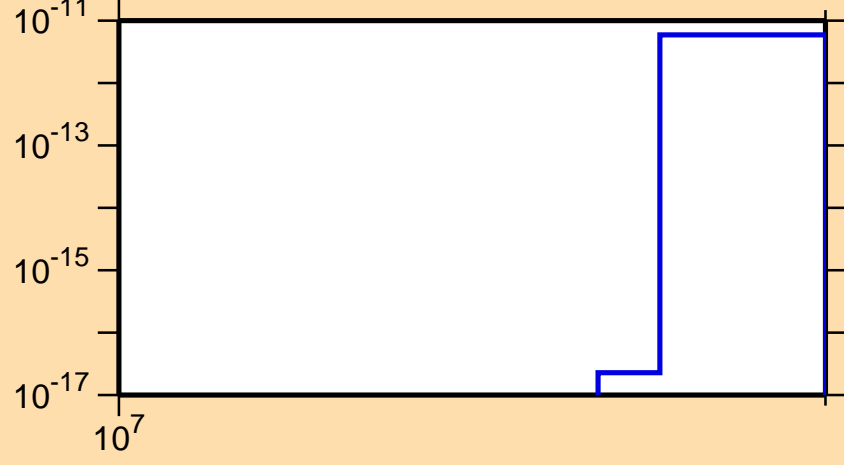
\sigma vs. E for ^{200}\text{Pt}(n,2np)
