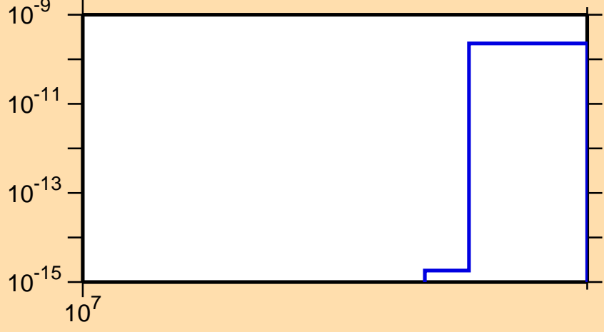
\sigma vs. E for ^{200}\text{Pt}(n,\text{nd})
