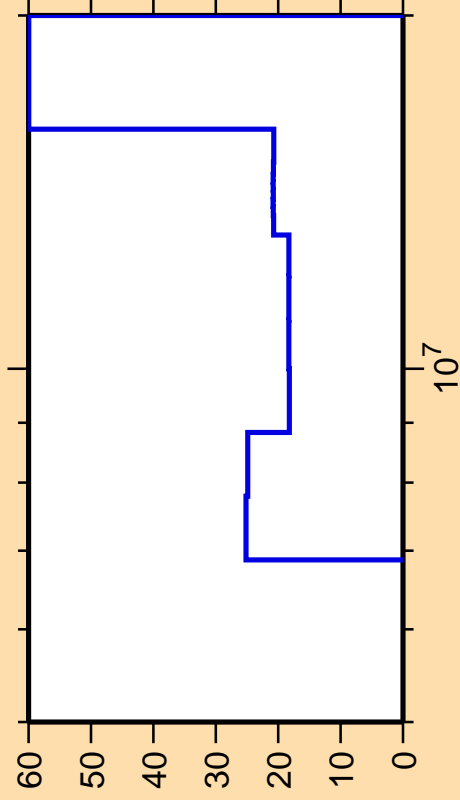
\Delta\sigma/\sigma vs. E for ^{200}\text{Pt}(n,2n)
