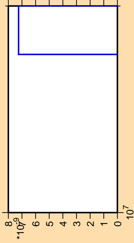
\Delta\sigma/\sigma vs. E for ^{200}\text{Pt} (mt 11)
