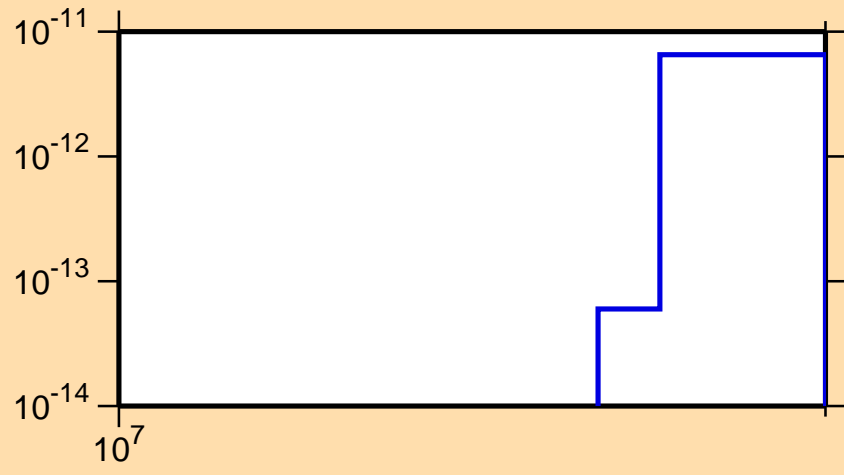
\sigma vs. E for ^{200}\text{Pt}(n,2n\alpha)
