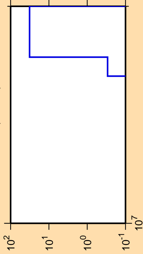
\Delta\sigma/\sigma vs. E for ^{200}\text{Pt}(n,2n\alpha)
