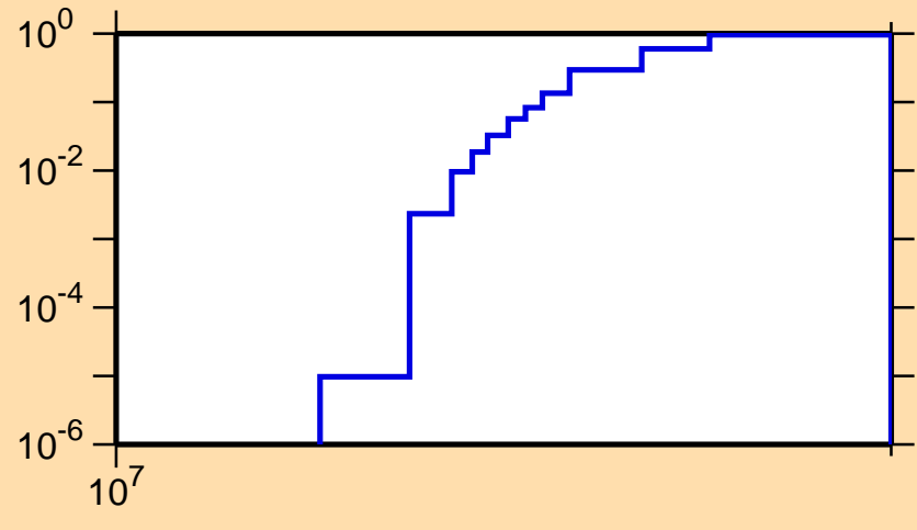
\sigma vs. E for ^{200}\text{Pt}(n,3n)
