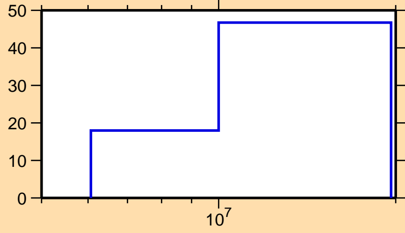
\Delta\sigma/\sigma vs. E for ^{200}\text{Pt}(n,ncont.)
