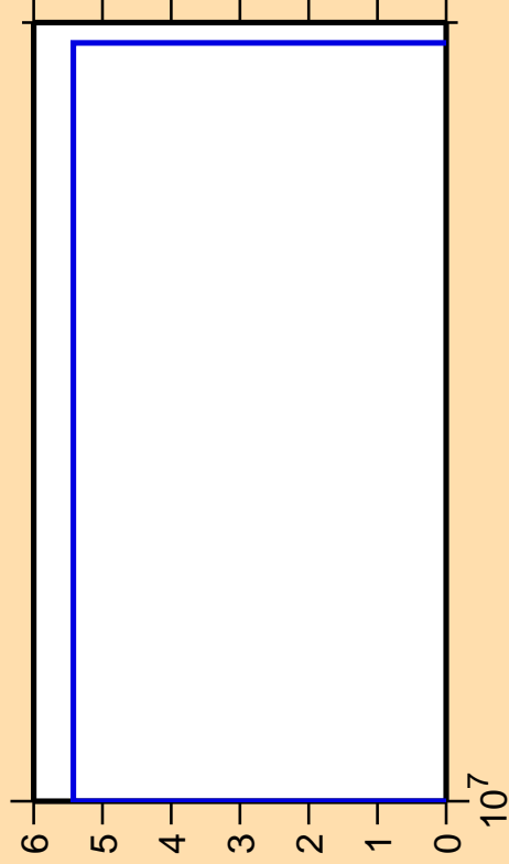
\Delta\sigma/\sigma vs. E for ^{200}\text{Pt}(n,nd)
