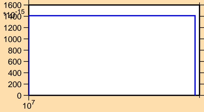
\sigma vs. E for ^{200}\text{Pt}(n,nd)
