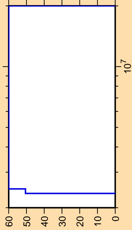
\Delta\sigma/\sigma vs. E for ^{200}\text{Pt}(n,\gamma)
