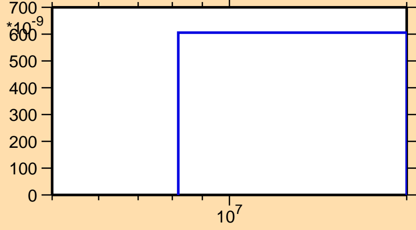
\sigma vs. E for ^{200}\text{Pt}(n,t)
