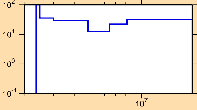
\Delta\sigma/\sigma vs. E for ^{200}\text{Pt}(n,n\text{cont.})
