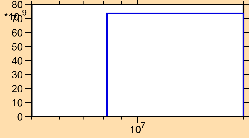
\sigma vs. E for ^{200}\text{Pt}(n,\alpha)
