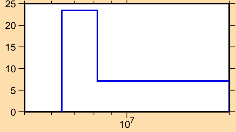
\Delta\sigma/\sigma vs. E for ^{200}\text{Pt}(n,el.)
