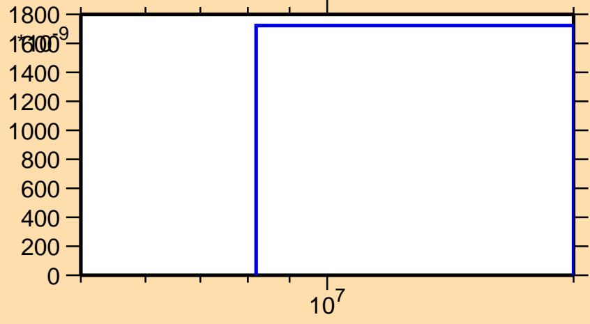
\sigma vs. E for ^{200}\text{Pt}(n,np)
