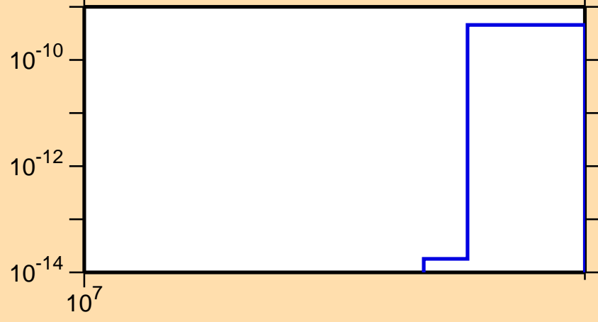
\sigma vs. E for ^{202}\text{Pt}(n,nt)
