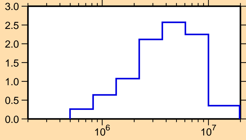
\sigma vs. E for ^{202}\text{Pt}(n,\text{inel.})
