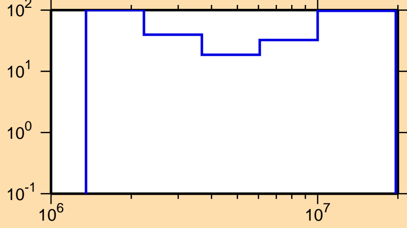
\Delta\sigma/\sigma vs. E for ^{202}\text{Pt}(n,n\text{cont.})
