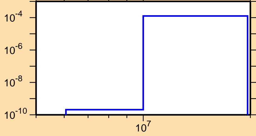
\sigma vs. E for ^{202}\text{Pt}(n,p)
