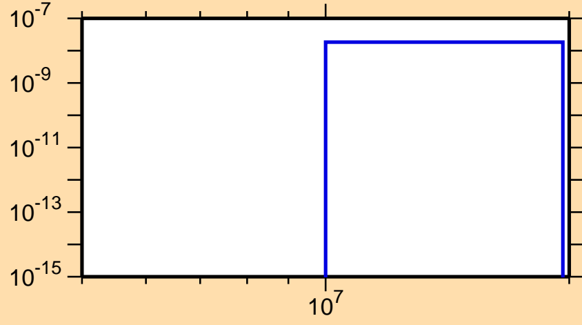
\sigma vs. E for ^{202}\text{Pt}(n,n\alpha)
