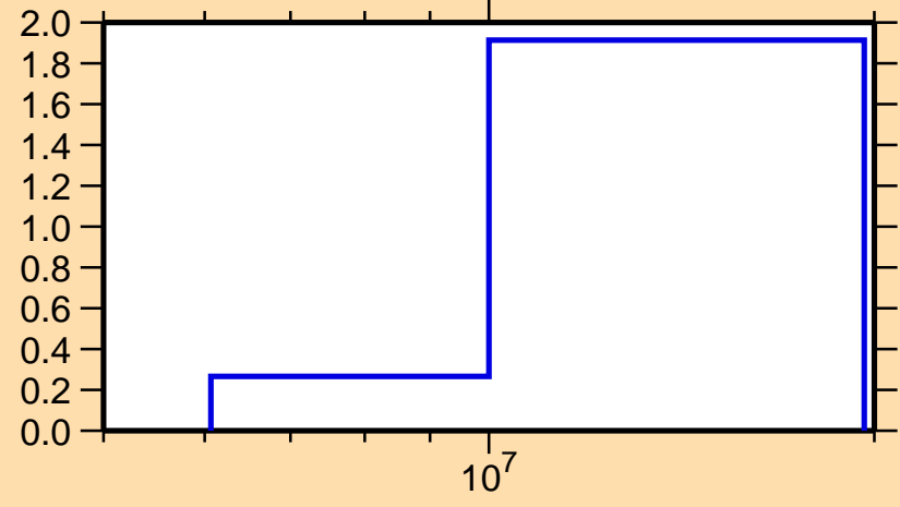
\sigma vs. E for ^{202}\text{Pt}(n,2n)
