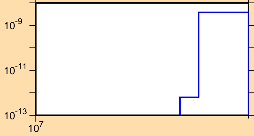
\sigma vs. E for ^{203}\text{Pt}(n,nt)
