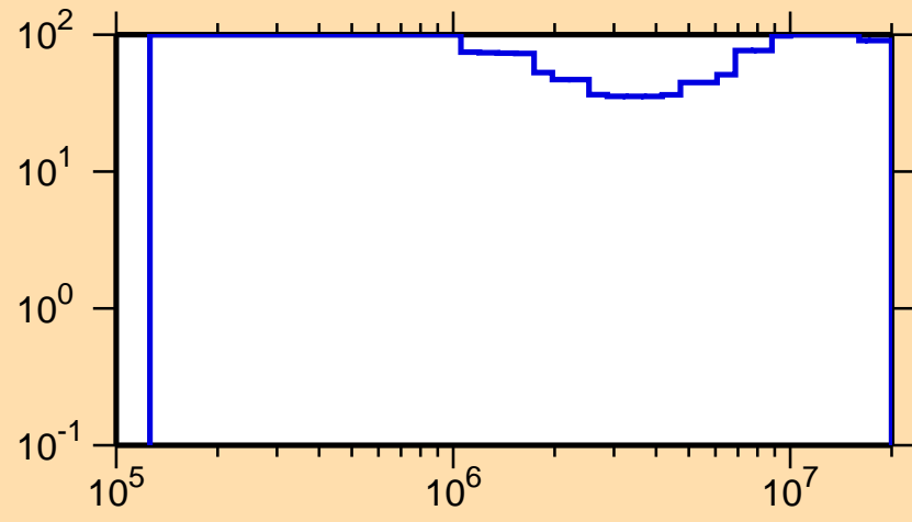
\Delta\sigma/\sigma vs. E for ^{203}\text{Pt}(n,n\text{cont.})
