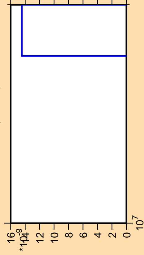
\Delta\sigma/\sigma vs. E for ^{203}\text{Pt} (mt 11)
