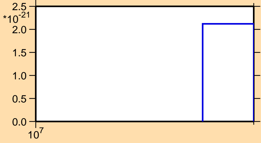
\sigma vs. E for ^{203}\text{Pt} (mt 11)
