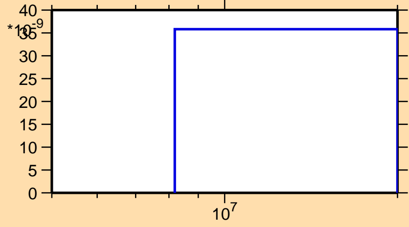
\sigma vs. E for ^{203}\text{Pt}(n,n\alpha)
