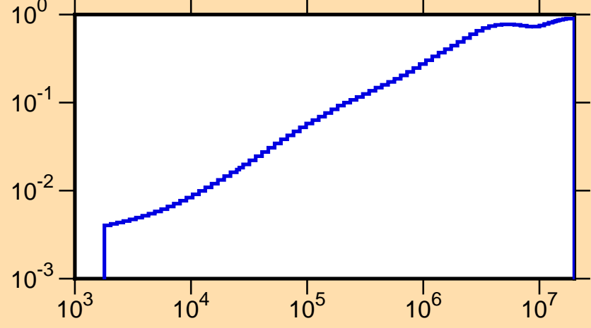
\mu vs. E for ^{205}\text{Pt}(\text{mt251})
