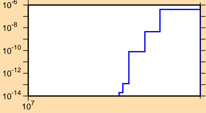
\sigma vs. E for ^{205}\text{Pt}(n,\text{nd})
