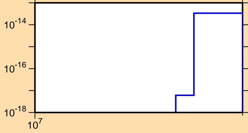
\sigma vs. E for ^{206}\text{Pt}(n,3n\alpha)
