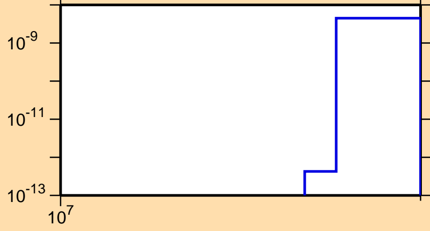
\sigma vs. E for ^{206}\text{Pt}(n,2np)
