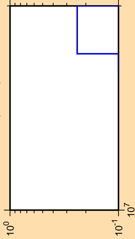
\Delta\sigma/\sigma vs. E for ^{206}\text{Pt}(n,3n\alpha)
