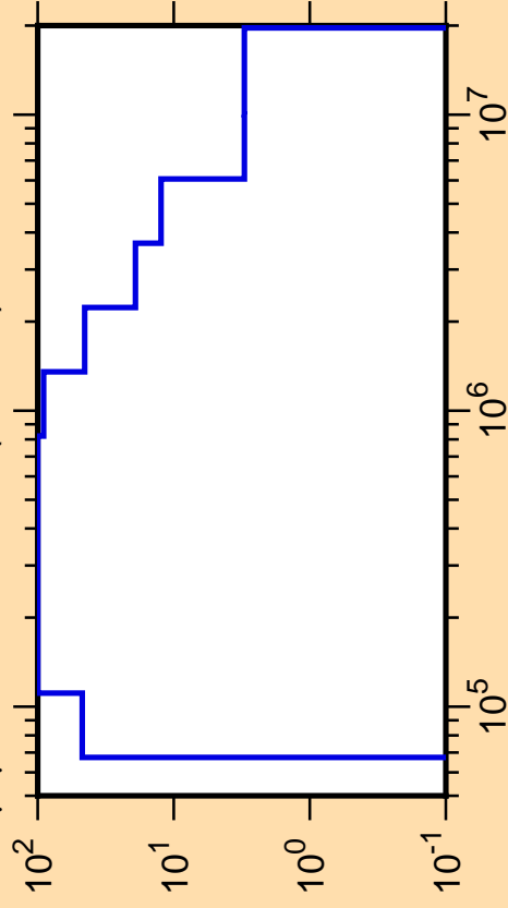
\Delta\mu/\mu vs. E for ^{206}\text{Pt}(\text{mt251})
