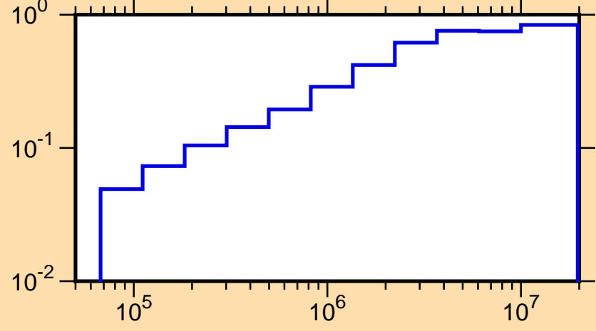
\mu vs. E for ^{206}\text{Pt}(\text{mt251})
