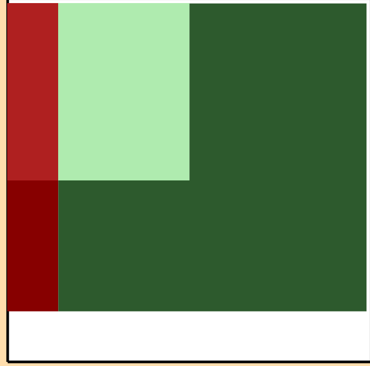
\Delta\sigma/\sigma vs. E for ^{206}\text{Pt}(n,\gamma)
