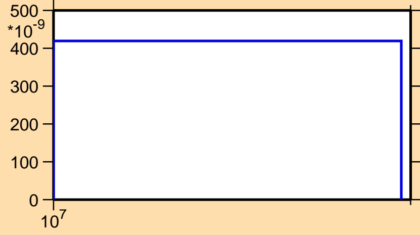
\sigma vs. E for ^{206}\text{Pt}(n,d)
