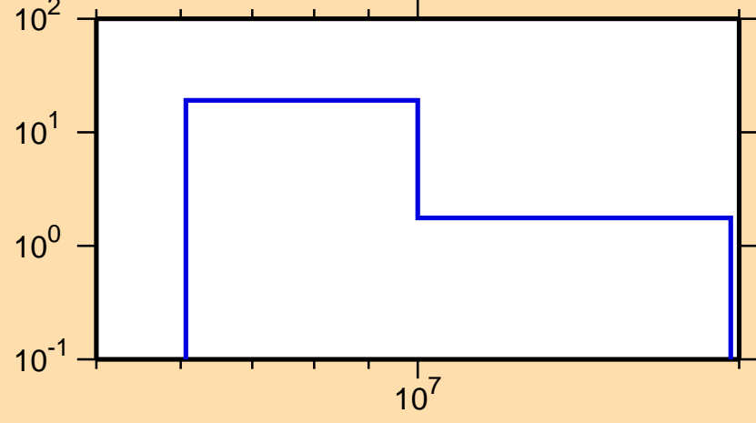
\Delta\sigma/\sigma vs. E for ^{206}\text{Pt}(n,\text{tot.})
