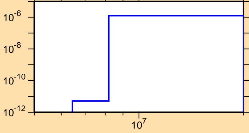
\sigma vs. E for ^{206}\text{Pt}(n,\alpha)
