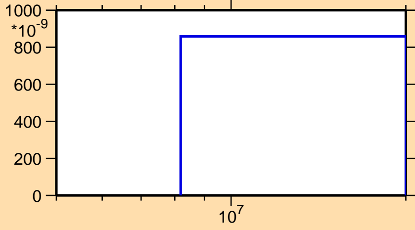
\sigma vs. E for ^{206}\text{Pt}(n,\alpha)
