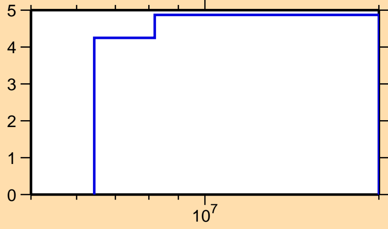
\Delta\sigma/\sigma vs. E for ^{206}\text{Pt}(n,\text{nonel.})
