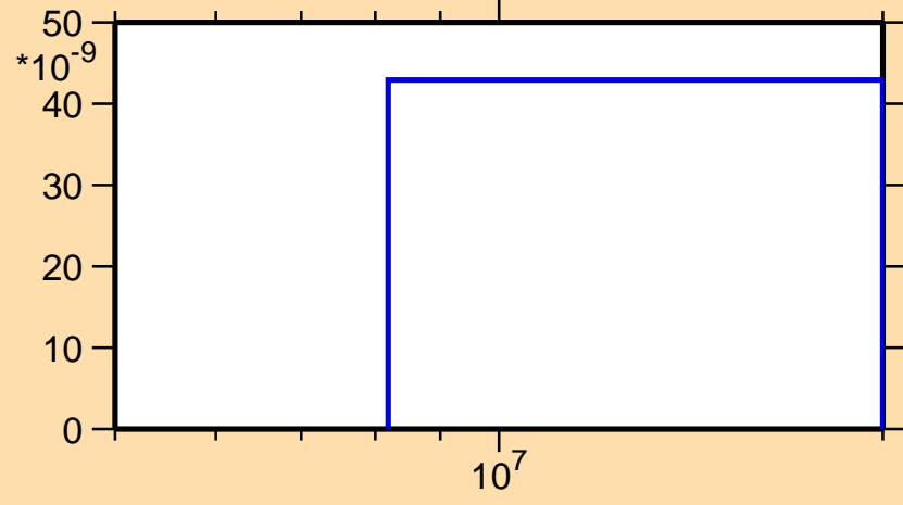
\sigma vs. E for ^{206}\text{Pt}(n,nt)
