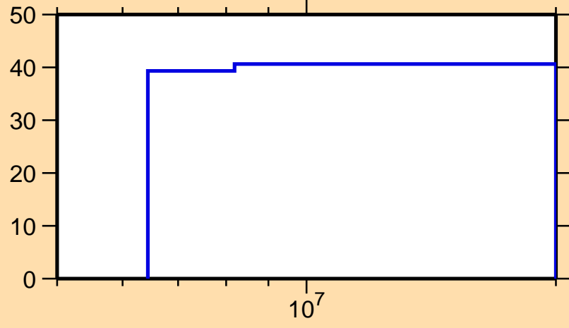
\Delta\sigma/\sigma vs. E for ^{206}\text{Pt}(n,ncont.)
