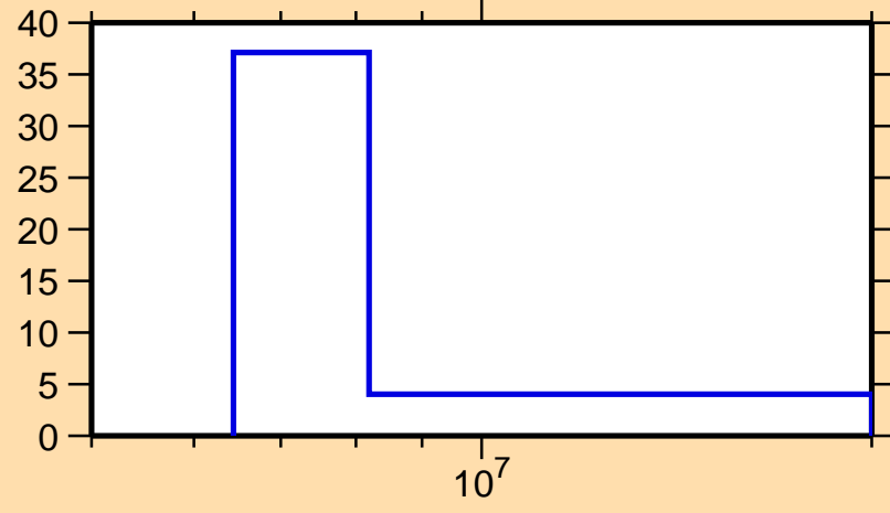
\Delta\sigma/\sigma vs. E for ^{206}\text{Pt}(n,el.)
