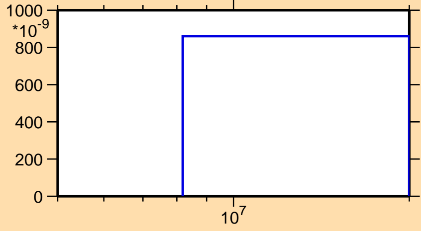
\sigma vs. E for ^{206}\text{Pt}(n,np)
