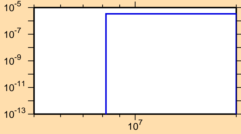
\sigma vs. E for ^{206}\text{Pt}(n,p)
