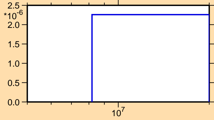
\sigma vs. E for ^{206}\text{Pt}(n,t)
