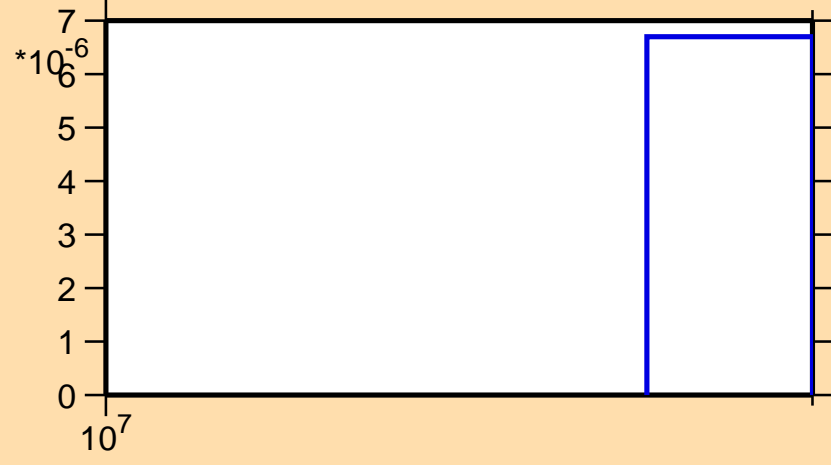
\sigma vs. E for ^{207}\text{Ra}(n,3n)
