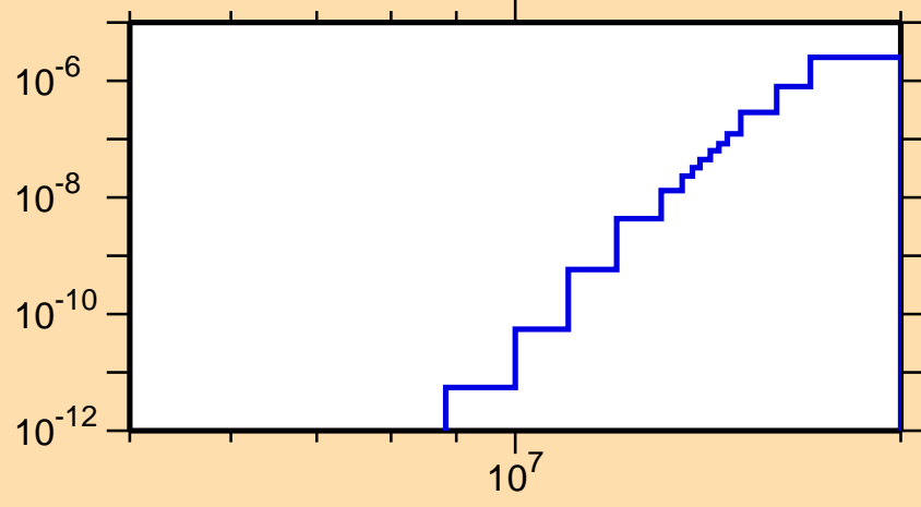
\sigma vs. E for ^{207}\text{Ra}(\text{mt } 45)
