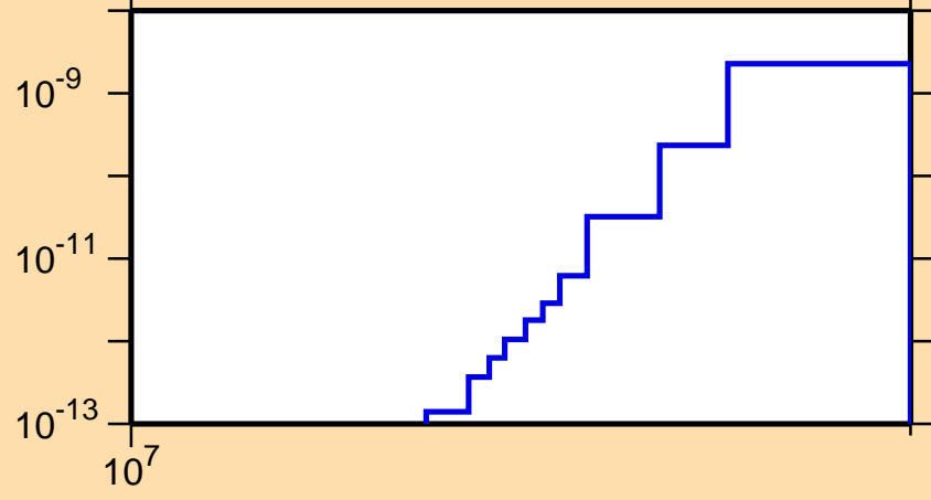
\sigma vs. E for ^{207}\text{Ra}(\text{mt } 34)
