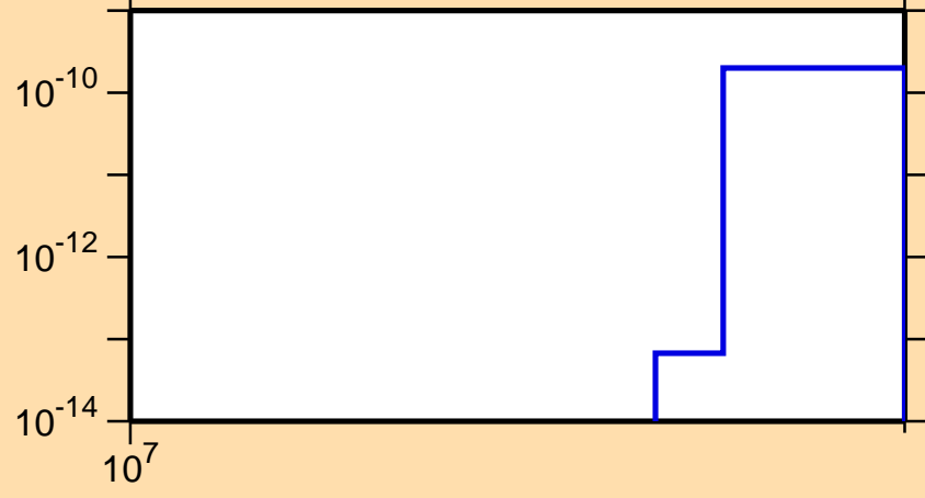
\sigma vs. E for ^{207}\text{Ra}(n,nt)
