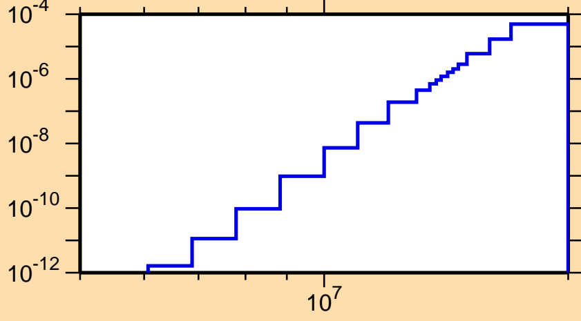
\sigma vs. E for ^{207}\text{Ra}(n,\text{He3})
