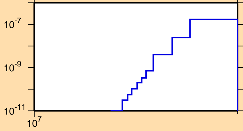
\sigma vs. E for ^{207}\text{Ra}(n,\text{pt})
