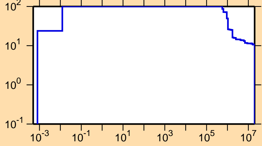
\Delta\sigma/\sigma vs. E for ^{207}\text{Ra}(n,\text{nonel.})
