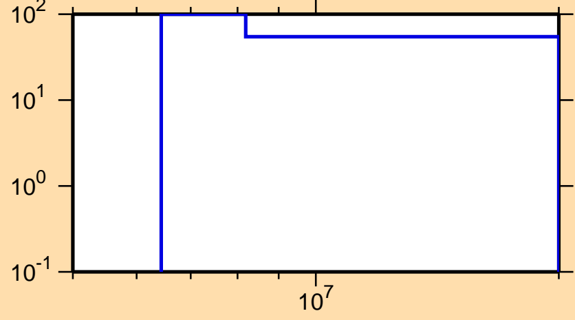
\Delta\sigma/\sigma vs. E for ^{207}\text{Ra}(n,2n)
