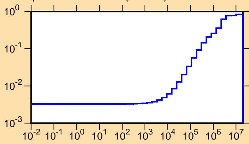
\mu vs. E for ^{208}\text{Ra}(\text{mt251})
