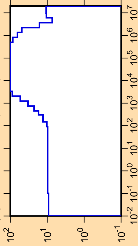
\Delta\mu/\mu vs. E for ^{208}\text{Ra}(\text{mt251})
