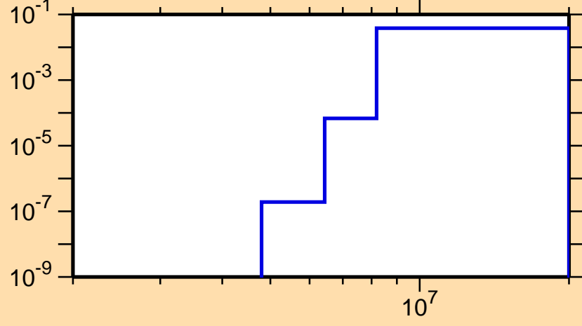
\sigma vs. E for ^{208}\text{Ra}(n,np)
