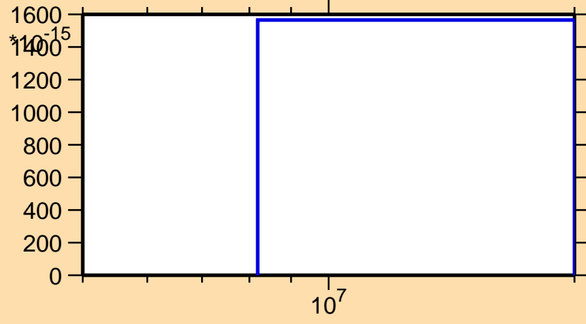
\sigma vs. E for ^{208}\text{Ra}(\text{mt } 34)
