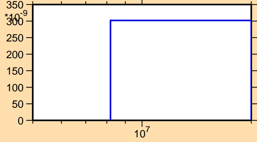
\sigma vs. E for ^{208}\text{Ra}(n,2np)
