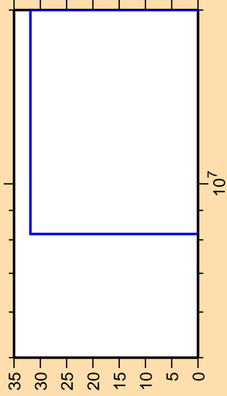
\Delta\sigma/\sigma vs. E for ^{208}\text{Ra}(n,n_1)
