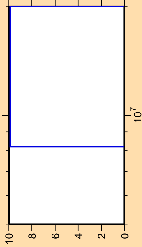
\Delta\sigma/\sigma vs. E for ^{208}\text{Ra}(\text{mt } 34)
