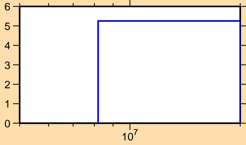
\Delta\sigma/\sigma vs. E for ^{208}\text{Ra}(n,\text{tot.})
