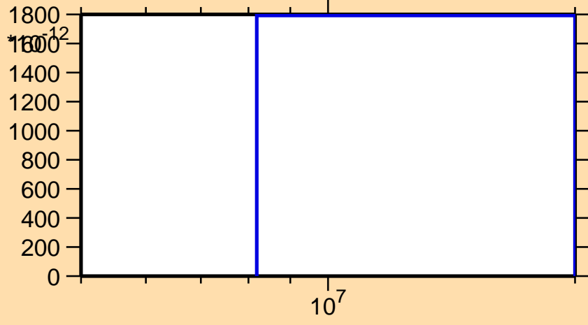
\sigma vs. E for ^{208}\text{Ra}(n,\text{nd})
