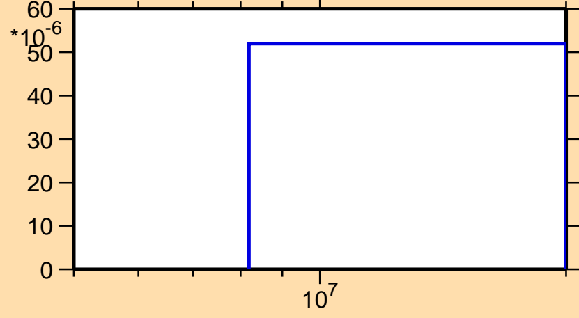
\sigma vs. E for ^{208}\text{Ra}(n,t)
