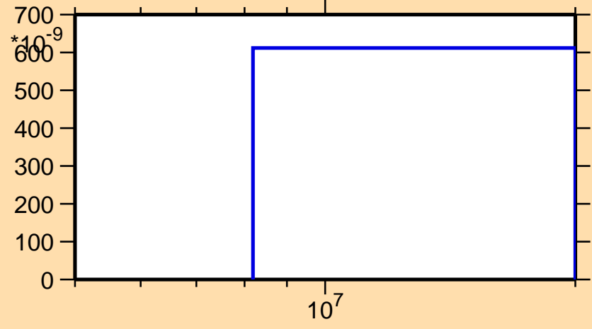
\sigma vs. E for ^{208}\text{Ra}(n,2n\alpha)
