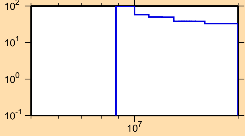
\Delta\sigma/\sigma vs. E for ^{210}\text{Ra}(n,2n)
