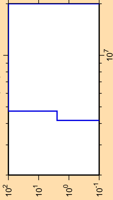
\Delta\sigma/\sigma vs. E for ^{210}\text{Ra}(n,d)
