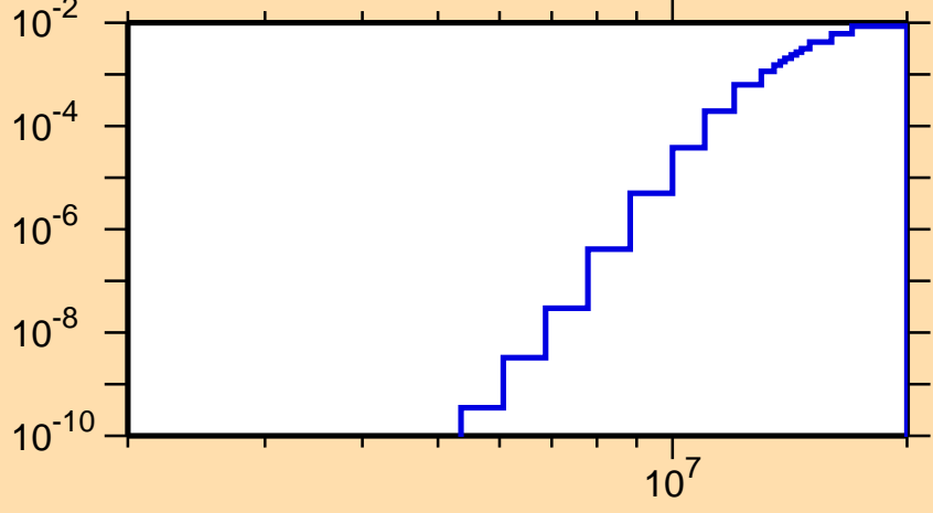
\sigma vs. E for ^{210}\text{Ra}(n,d)
