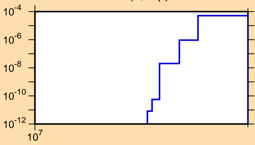
\sigma vs. E for ^{210}\text{Ra}(n,2np)
