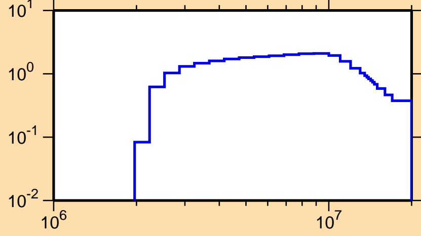
\sigma vs. E for ^{210}\text{Ra}(n,\text{inel.})
