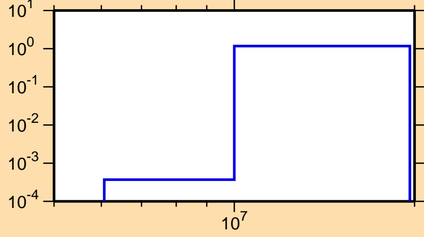
\sigma vs. E for ^{210}\text{Ra}(n,2n)
