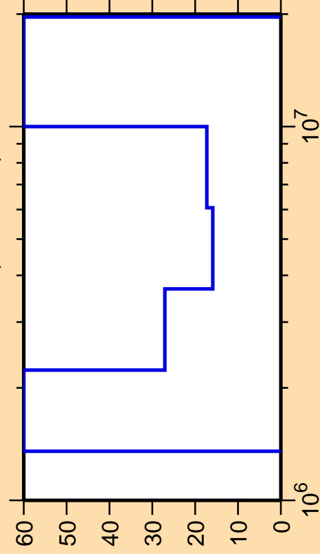
\Delta\sigma/\sigma vs. E for ^{210}\text{Ra}(n,\text{ncont.})
