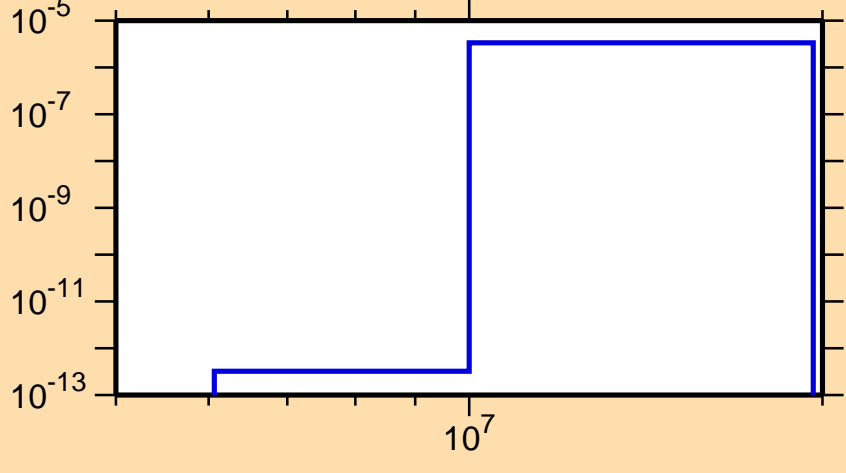
\sigma vs. E for ^{210}\text{Ra}(n,2n\alpha)
