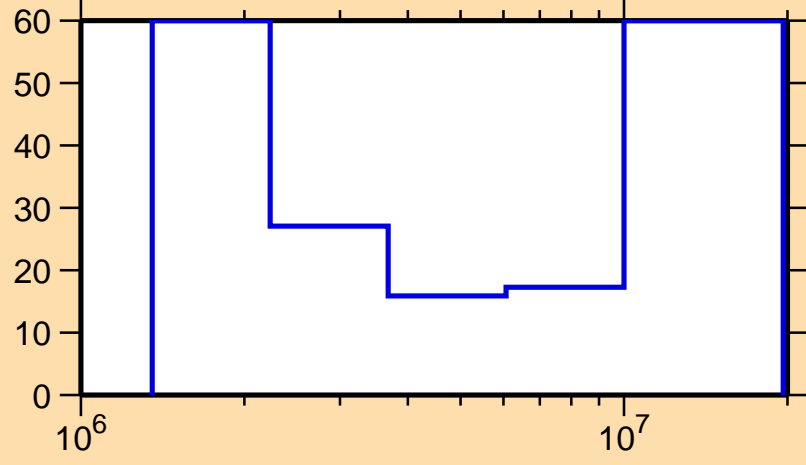
\Delta\sigma/\sigma vs. E for ^{210}\text{Ra}(n,n\text{cont.})
