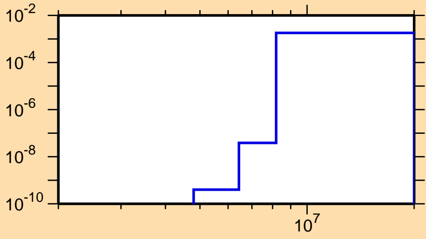
\sigma vs. E for ^{210}\text{Ra}(n,d)
