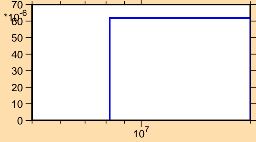
\sigma vs. E for ^{210}\text{Ra}(n,t)
